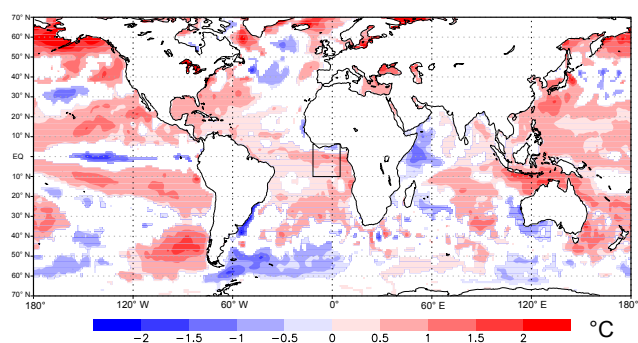
Figure 2. Global SST anomalies for June–July 2016 (°C). Basis is the Reynolds Optimal Interpolated SST v2 dataset and anomalies are relative to 1981–2016. Only anomalies above the 95 % confidence level based on a two-sided Student's t test are plotted. The black box marks the area used for Fig. 3.
