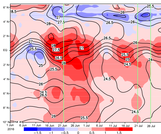
Figure 3. Daily SST behaviour over the eastern tropical Atlantic during June–July 2016. SSTs (°C) are averaged between 10° W and 4° E (see box in Fig. 2) and shown as absolute values (lines) and anomalies (shading). Basis is the Reynolds Optimal Interpolated SST dataset and anomalies are relative to 1981–2016 as in Fig. 2. Only values greater than the SST Reynolds daily error estimation are plotted. The four phases of the DACCIWA campaign are marked with thin green lines.
