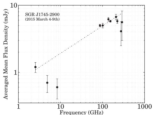
Figure 3. Average spectrum of SGR J1745–2900 from the observations. The dash–dotted line shows the spectral index fit using a single power law. The mean spectral index obtained is \langle \alpha \rangle = +0.4 \pm 0.2 . Error bars are 2\sigma .
