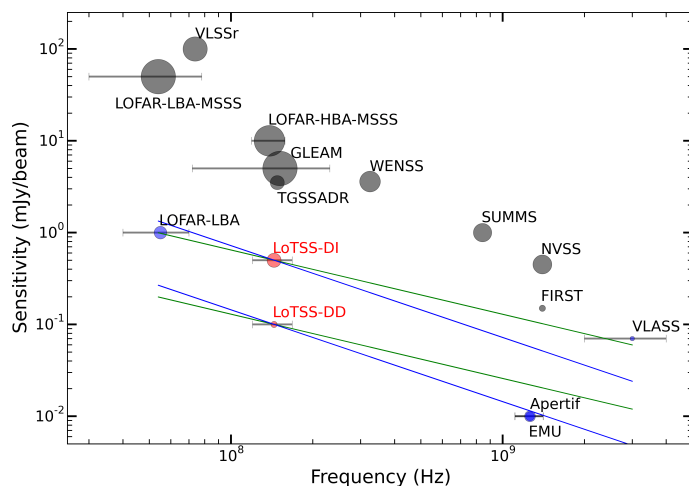
Fig. 1. A summary of the sensitivity, frequency and resolution of a selection of recent and planned large-area radio surveys (see also Table 1). The size of the markers is proportional to the square root of the survey resolution. Grey, blue and red markers show the ongoing/completed surveys, forthcoming surveys, and the LOFAR HBA surveys respectively. The horizontal lines show the frequency coverage for surveys with large fractional bandwidths ( > 0.2 ). The green sloping lines show the sensitivity that is equivalent to that achieved in the LoTSS direction-dependent (DD) calibrated and direction-independent (DI) images for typical radio sources with a spectral index \sim -0.7 . Similarly, the blue sloping lines show the equivalent sensitivity to steep spectrum sources with a spectral index \sim -1.0 .
