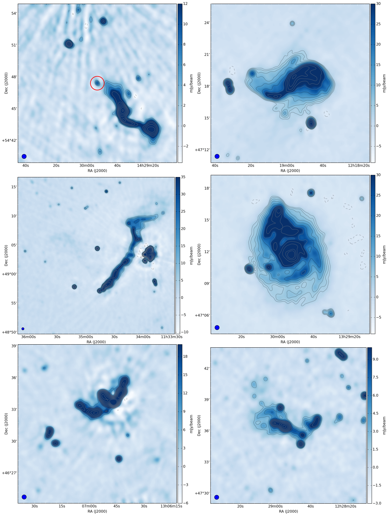
Fig. 15. A sample of rare objects whose low-frequency emission we have characterised in the 25'' resolution preliminary data release images which are now available for download in FITS format. Clockwise from top left: the z = 6.21 quasar J1429+5447 (circled); the nearby galaxies M 106 and M 51; the merging galaxy clusters Abell 1550 and Abell 1682; the Mpc-scale tailed radio galaxy IC 711 that resides in the galaxy cluster Abell 1314. The contours and colour scale vary between images and were chosen to best emphasise the structure of each object. The synthesised beam is shown in the bottom left corner of each image.
