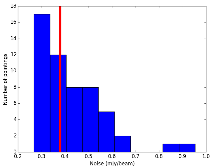
Fig. 10. A histogram showing the noise estimates from the direction-independent calibrated LOFAR images. The median noise level (shown by the vertical red line) for the 54 HETDEX pointings is 380 \mu\text{Jy}/\text{beam} and the noise levels range from 270 \mu\text{Jy}/\text{beam} to 960 \mu\text{Jy}/\text{beam} .
