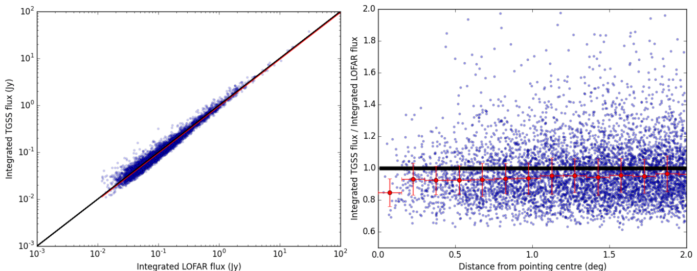
Fig. 9. A comparison between the LOFAR integrated flux density measurements and the TGSS measurements with each cross-matched isolated compact source shown with a solid circle. On the left is a comparison of the integrated flux densities. The solid black lines show a 1:1 ratio of the integrated flux densities and the solid red line shows the median ratio between the integrated flux density measurements. On the right is a comparison of the integrated flux density ratio as a function of distance from the LOFAR pointing centre. The red symbols indicate the median within bins of distance, with the vertical error bars showing the median absolute deviation (MAD) value for each bin and the horizontal error bars giving the bin width. The median value of the TGSS integrated flux density divided by the LOFAR integrated flux density is 0.95.
