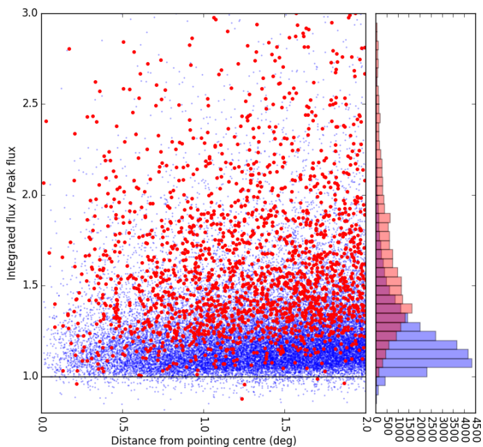
Fig. 7. The ratio of the integrated flux density to peak brightness for compact sources in all 54 LOFAR pointings. The seven pointings identified as having particularly poor ionospheric conditions are shown in red and the remaining 54 pointings are shown in blue. The histogram of the red points has been multiplied by a factor of 10 for display purposes.
