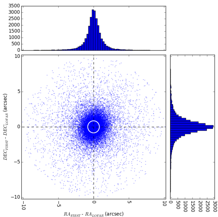
Fig. 8. The residual RA and Dec offsets for LOFAR detected sources matched with their FIRST counterparts. The ellipse shows the standard deviation of the RA and Dec offsets ( 1.65'' and 1.70'' respectively) and is centred on the mean offset which is zero in both RA and Dec. The points show the RA and Dec offsets for each of the matched sources. The histograms show the number of sources at different RA and Dec offsets.
