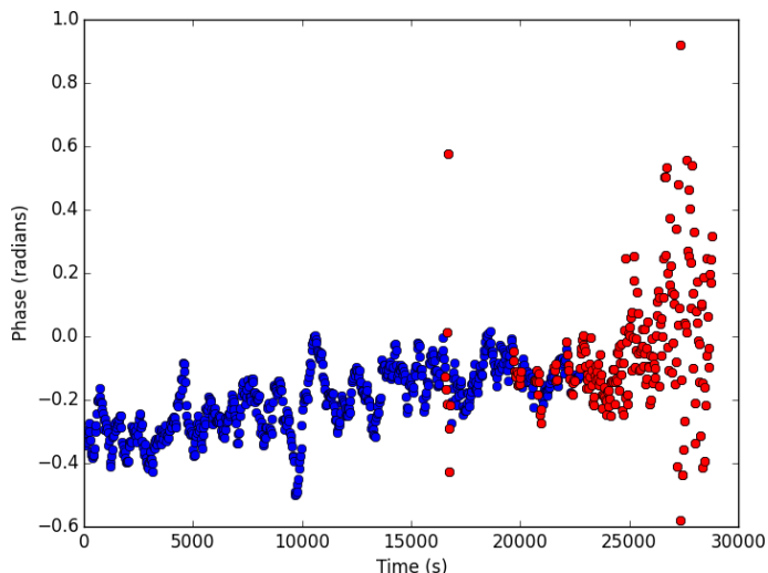
Fig. 6. The phase solutions for station CS401HBA1 using station CS032HBA1 as a phase reference for a LoTSS dataset are shown in blue (CS032HBA1 is the closest station to CS401HBA1 at a distance of 584 m). The red points show the time periods where the phase solutions indicate poor ionospheric conditions (see Section 4.1) and these time periods are subsequently flagged.
