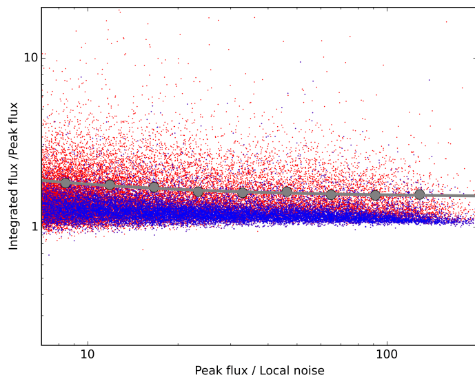
Fig. 11. The ratio of the integrated flux density to peak brightness for sources in the preliminary data release catalogue as a function of the signal-to-noise ratio. Sources with a size of less than 5'' in the FIRST catalogue are shown in blue and all other sources are shown in red. The large dots indicate the boundary that contains 95% of the compact FIRST detected sources and the line shows the best fit to this boundary which is given by \frac{S_{\text{int}}}{S_{\text{peak}}} = 1.50 + 1.78 \left( \frac{S_{\text{peak}}}{\text{RMS}} \right)^{-0.78} .
