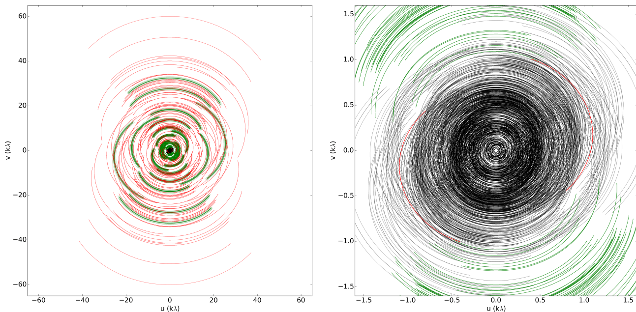
Fig. 2. The monochromatic uv plane coverage of a typical 8 hr 150 MHz LoTSS observation around declination +55^\circ excluding the international stations. On the left is the full uv coverage and on the right we show the dense uv -coverage in the inner region of the uv -plane. Here the monochromatic coverage has been presented for display purposes but the full bandwidth used in each observation is 48 MHz, which corresponds to a fractional bandwidth of \sim 1/3 , and this provides considerable additional filling of the uv -plane. The uv points are colour coded according to the type of stations that make up each baseline. Those containing only core stations, remote stations, or a combination of the two are shown in black, red, and green respectively.
