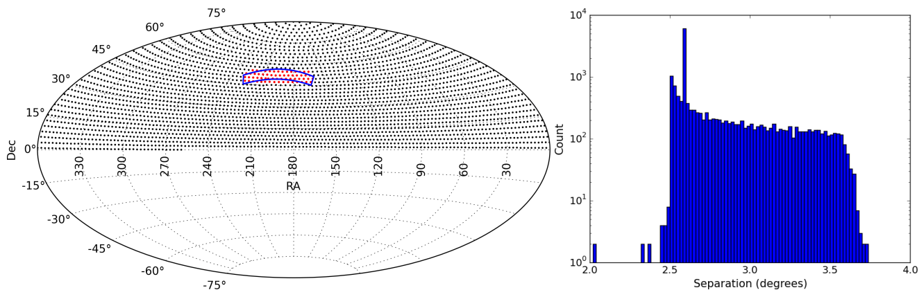
Fig. 3. The left panel shows the LoTSS pointing grid which follows a spherical spiral structure. The region highlighted in blue is the HETDEX Spring Field. The red points show the LOFAR pointings that are presented in this publication and the black points show the rest of the survey grid. The right panel shows a histogram of the separation of the six nearest neighbours to each of the 3170 pointings in the survey grid excluding the edge pointings close to declination zero. A log scale is used on the y-axis in order to clearly display the full variation of pointing separations. The mean separation of pointings is 2.80^\circ but the distribution is highly peaked around the median separation of 2.58^\circ . In total, 65% of pointings have all six nearest neighbours within 2.80^\circ and 98% have at least four neighbouring pointings within 2.80^\circ . Note that the panel on the right was created from a grid with a complete spherical spiral structure and ignores the 42 test pointings that were conducted with a slightly different tiling strategy.
