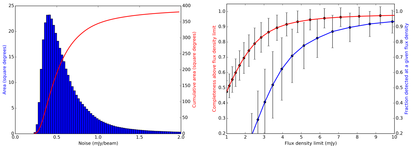
Fig. 12. Left: The estimated noise variations on the direction-independent calibrated mosaiced images within the 381 square degree region encompassed by the FWHM of the mosaiced pointings. The red line shows the cumulative area of the mosaiced region that has a estimated noise less than a given value. The histogram shows the distribution of noise estimates within the mosaiced region. Right: The estimated cumulative completeness of the preliminary data release catalogue (red) and the fraction of simulated sources that are detected as a function of flux density (blue). A large number of sources were injected during the completeness simulations and as a consequence the poissonian errors are negligible. However, the spatial variation in noise is substantial and the error bars show the standard deviation of the measurements as a function of position.
