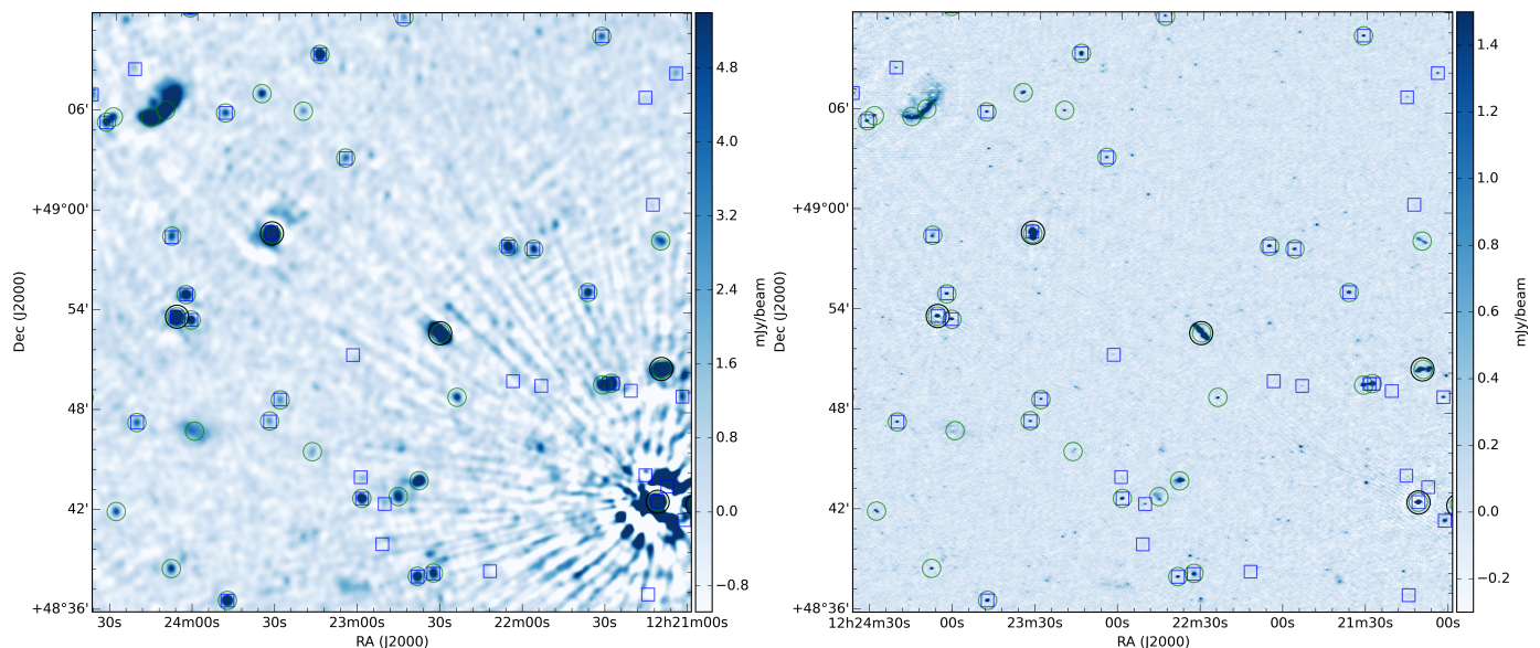
Fig. 13. A comparison between the direction-independent calibrated images and those we expect from direction-dependent calibration. On the right the facet calibration method has been used to create a high resolution, high fidelity, approximately thermal noise limited image and on the left is the same region in our direction-independent calibrated images. The colour scales on both images is between -3 and 10 times the noise where the direction-independent calibrated image noise is 360 \mu\text{Jy}/\text{beam} and the facet calibrated image noise is 100 \mu\text{Jy}/\text{beam} . The green circles show the positions of sources detected at seven times the noise in the direction-independent LOFAR image. The larger black circles and the blue squares indicate entries in the TGSS and FIRST catalogues respectively.
