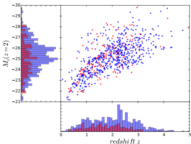
Fig. 14. The distribution of quasars in the magnitude-redshift space for the BOSS radio-loud quasars (Pâris et al. 2014) inside the survey footprint. Whilst 551 radio-quasars are detected in both the FIRST and LOFAR images (blue circles), LOFAR is able to detect a further 191 that are not detected in FIRST (red circles). The absolute magnitude in the i band at z = 2 M_i(z = 2) is calculated using the K-correction from Richards et al. (2006). The left and bottom panels show the M_i(z = 2) and redshift histograms.
