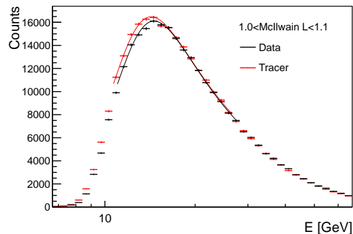
FIG. 17. Measured count spectrum (black) of primary CREs after removal of secondary electrons for the McIlwain L interval [1.0, 1.1], and the count spectrum predicted by tracer . The latter is normalized so that its integral above 20 GeV is the same as in the data.
