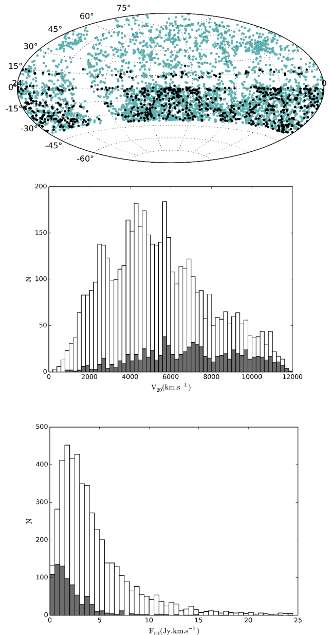
Fig. 1. General statistics of the KLUN HI catalog. Top : Aitoff projection of the KLUN composite Nançay HI-data catalog (cyan dots: Theureau et al. (1998a), Paturol et al. (2003b), Theureau et al. (2005), Theureau et al. (2007); black dots: the galaxies added in this publication). Middle: distribution of radial velocities (optical convention) for the KLUN composite catalog (white columns) and this paper (gray columns). Bottom: distribution of beam-corrected HI-fluxes (same samples).
