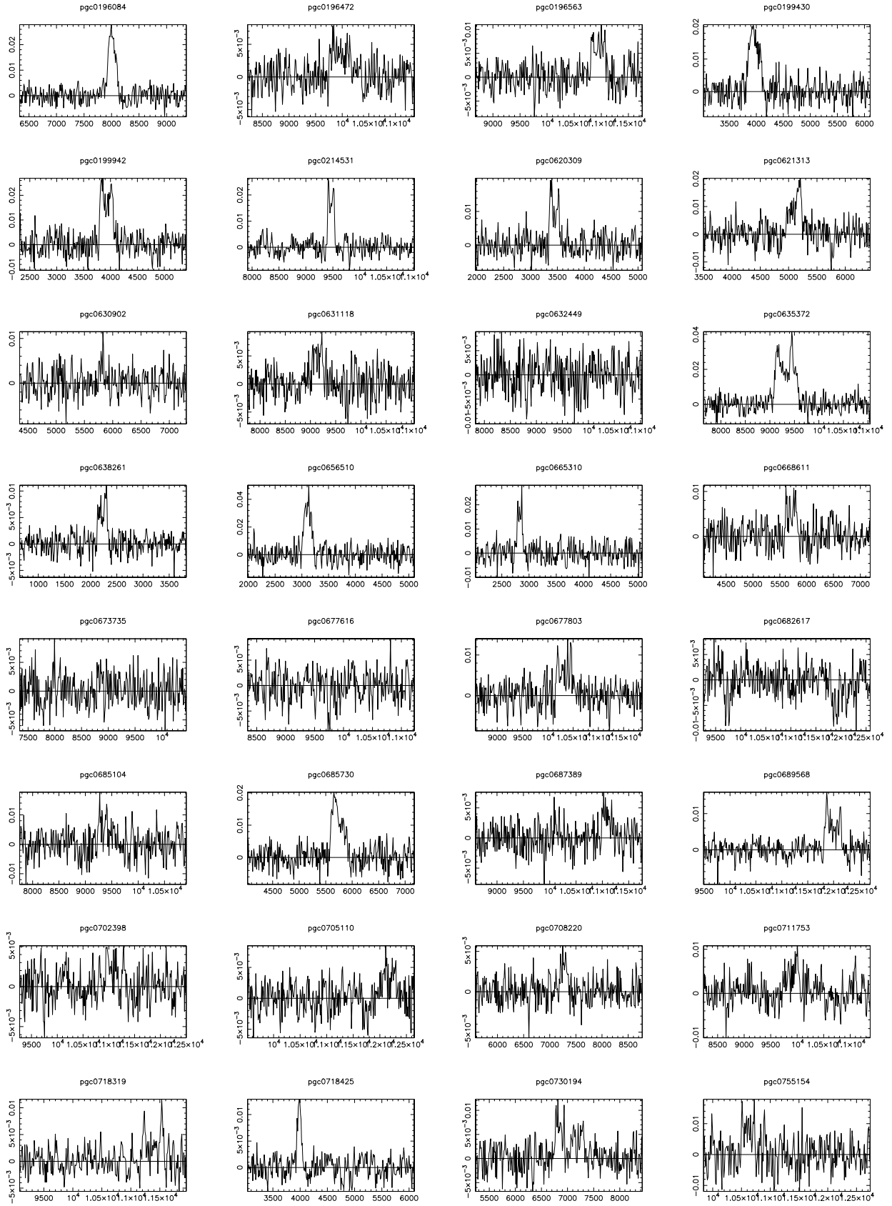
Fig. A.1. Fig. 2 x. HI profiles. Continued.
