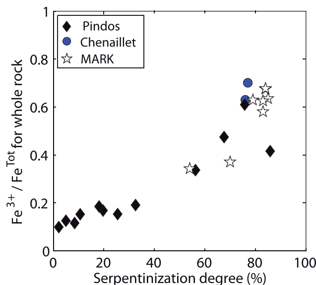
Figure 10. \text{Fe}^{3+} content in whole rock versus serpentinization degree (calculated from grain density). Data for Chenaillet are from Debret et al. [2014].
