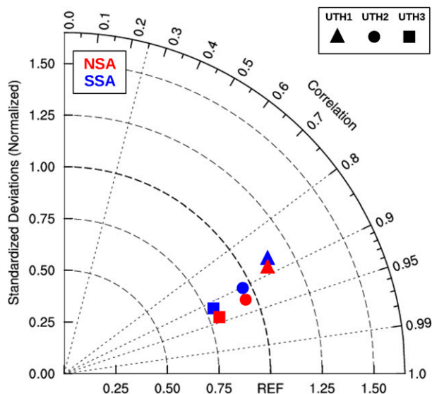
FIG. 3. Taylor diagram describing the similarities between the UTHs from SAPHIR and the UTH CDA over NSA (red), SSA (blue), and during OND 2011. UTH CDA is considered as the reference (indicated by REF). Correlations are significant at 0.25 according to a 1% risk t test.
