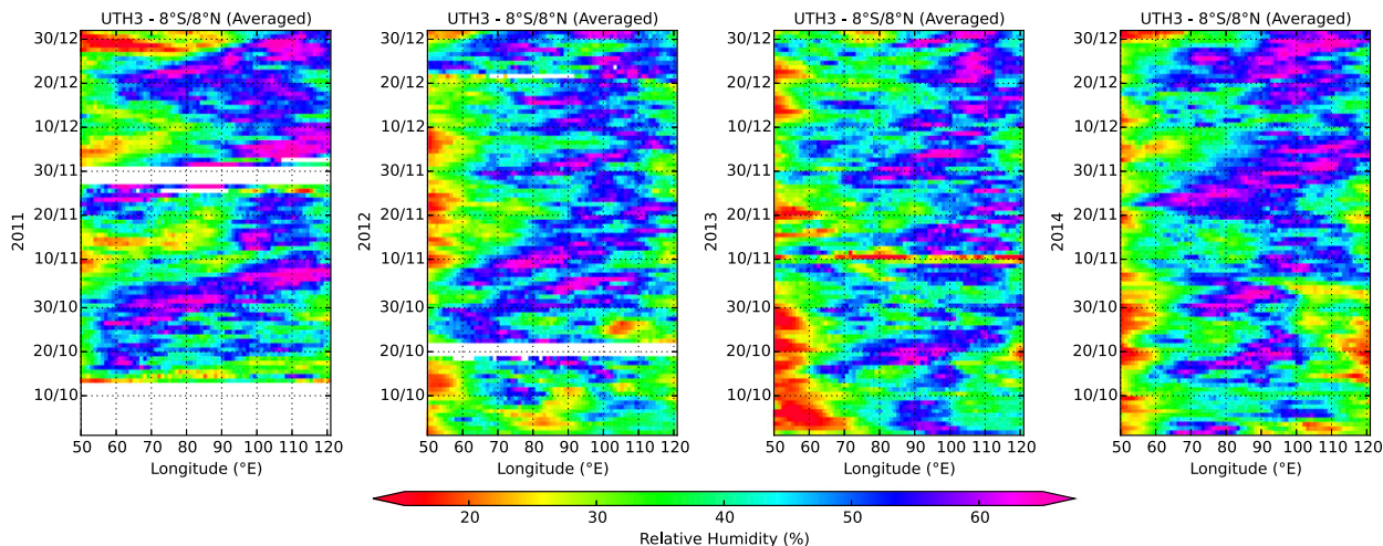
FIG. 4. Longitude–time Hovmöller diagrams of UTH3 from SAPHIR (remapped into 1° × 1 day) covering October–December from (far left) 2011 to (far right) 2014. Time increases upward. Latitudes are averaged over the NSA–SSA limits (8°N–8°S).
