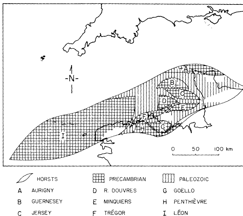
Figure 14. Schematic depiction of the structural units of the Domnonean Domain of the Armorican Massif (after Lefort 1965).
