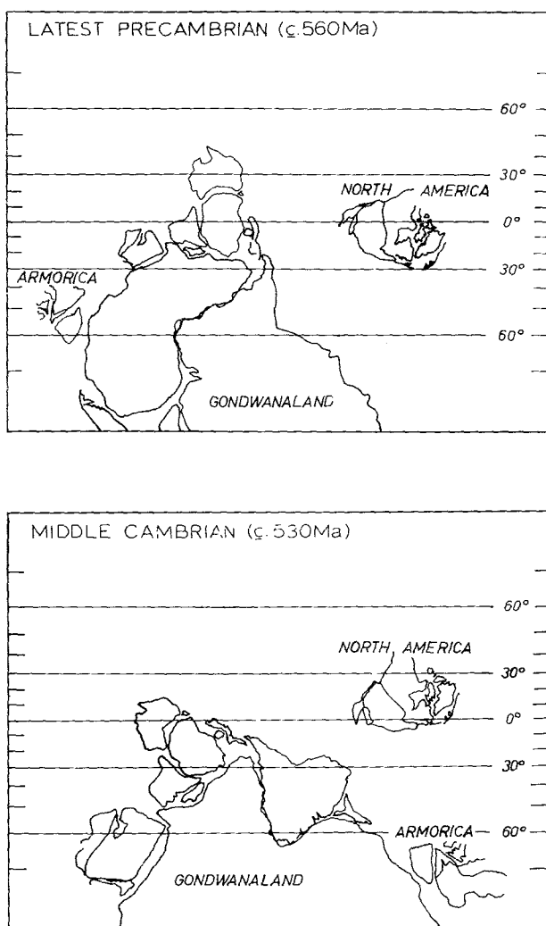
Figure 17. Mercator palaeolatitude reconstructions based on Latest Precambrian poles (UB, AS, BH, AV) and Middle Cambrian poles (LF, AD) of Table 4 for Gondwana, as well as on poles listed by Elston & Bressler (1977), Van der Voo, French & Williams (1976), and Watts (1979) for North America.
