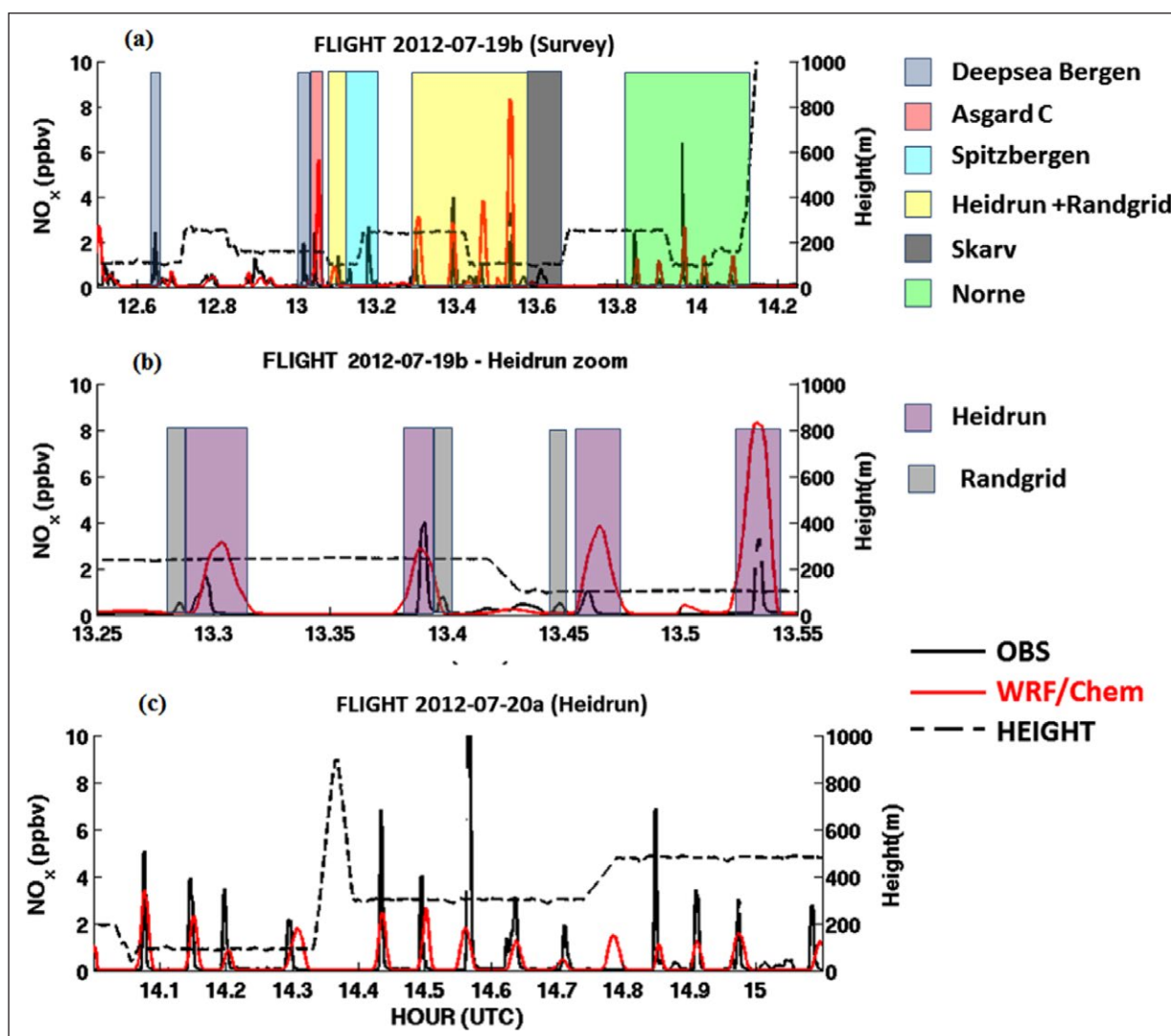
Figure 5: Comparison between observed and modeled \text{NO}_x and \text{O}_3 on 19 July 2012. Observed (black) and simulated (CTRL run red) time series of \text{NO}_x on 19 (a) and 20 (c) July 2012. The panel (b) is a zoom on the Heidrun and Randrid plume of the 19 July. Model simulations included emissions from the Asgard, Heidrun and Norne facilities (see text for details). DOI: https://doi.org/10.1525/elementa.124.f5
