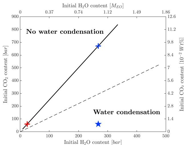
Figure 17. Water condensation diagram for the early Earth ( \alpha = 0.2 , D = 1 AU, young Sun) as a function of H_2O and CO_2 . Above the condensation limit (black line), CO_2 precludes the formation of a water ocean. The dashed line stands for a chondritic CO_2/H_2O ratio, the blue star represents the early Earth's position, and the crosses the critical volatile contents associated. Parameters used for the calculations are given in Table 2.
