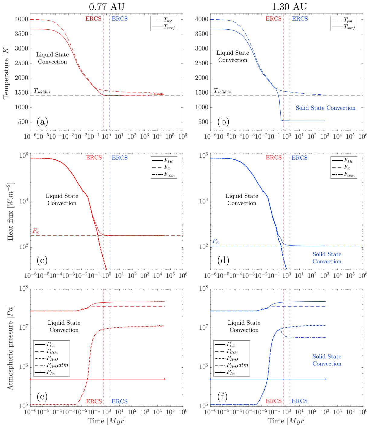
Figure 5. Thermal evolution of the magma ocean for two different distances from the Sun: 0.77 AU (a, c, and e, red) and 1.30 AU (b, d, and f, blue), grey atmosphere, without clouds, [H_2O]_{t_0} = 0.621 M_{E_0} , [CO_2]_{t_0} = 5 \times 10^{-2} wt %. ERCS is indicated by the vertical dotted lines. P_{H_2O\text{atm}} corresponds to the uncondensed H_2O partial pressure remaining in the atmosphere if condensation occurs at surface and stores water in the oceans (here a 480 m deep water ocean is formed at 1.30 AU). Corresponding thermal atmospheric profiles at ERCS are shown in Figure 4. Parameters used for the calculations are given in Table 2.
