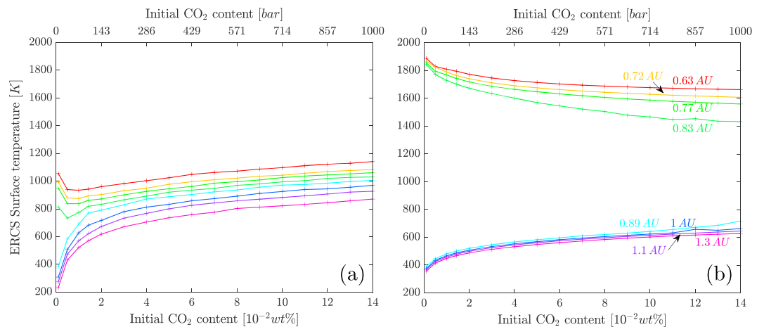
Figure 13. Surface temperatures obtained at ERCS for solar distances varying from 0.63 to 1.30 AU, initial CO 2 contents from 0.1 to 14 × 10 -2 wt % and initial water contents equal to (a) 0.031 M EO and (b) 1.243 M EO . Parameters used for the calculations are given in Table 2.
