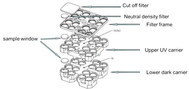
Fig. 40 EXPOSE-E integrated on the EuTEF platform before launch (Credit: ESA). The bottom two compartments and the lower half of next compartments contained the sample carriers (explosion drawing on the right, adapted, credit: Kayser-Threde) with the sample from ADAPT. Left vertical row is tray 1, open to space; middle vertical row is tray 2 with Mars conditions
