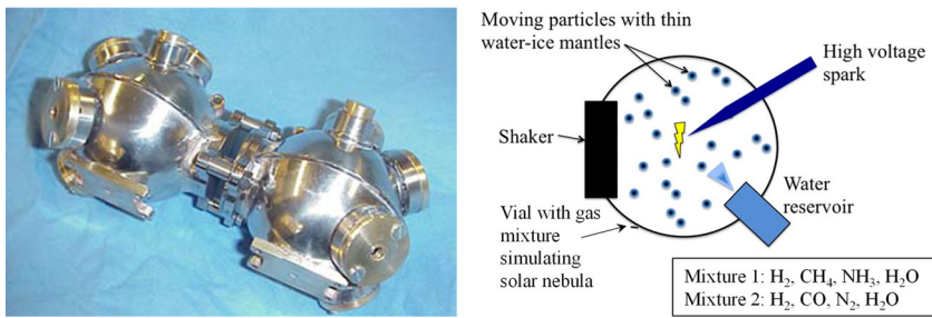
Fig. 33 Left : picture of a prototype of the MU experiment (Dual Vial Construction). Right : a representative diagram of the proposed MU experiment illustrating the water-ice coated particles, a high voltage spark discharge (energy source), a shaker to slowly move the particles in near-weightlessness and water reservoir system to inject water to coat the particles at the start of the experiment
