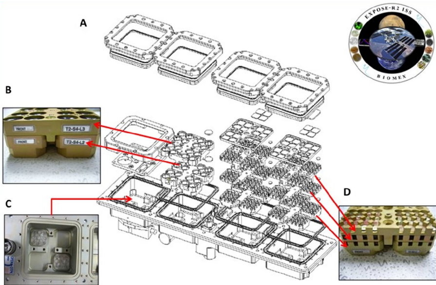
Fig. 43 Schematic illustration of the EXPOSE-R2/BIOMEX hardware: (A) overview on the compartments and the different sample holder levels (top layer: exposed directly to solar radiation, bottom layer space-dark control areas). (B) Compartment with place for 32 ( 2 \times 16 ) samples. It is divided into two parts with top (radiation exposure) and bottom layer (space-dark control). In the BIOMEX experiment one of this compartment type is exposed in addition to space/solar radiation to space vacuum and another compartment of this size is exposed to a Martian atmosphere. (C) Passive radiation detectors placed on the bottom of the samples. (D) Compartment with place for 192 ( 3 \times 64 ) samples. It is divided into three parts with top (radiation exposure) and two bottom layer (space-dark control). In the BIOMEX experiment this compartment is exposed in addition to space/solar radiation to the Martian atmosphere
