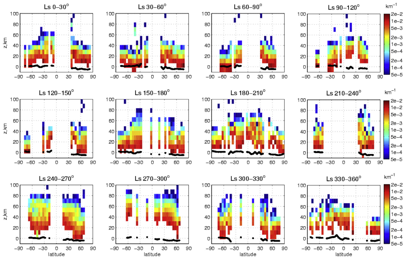
Fig. 9. Seasonal and spatial distribution of the extinction ( \text{km}^{-1} ) vertical profiles at 1094 nm averaged on a grid 30^\circ of L_s \times 5^\circ of latitude \times 6 km of altitude for 4 MY (MY27–31) from orbit 1200 to orbit 12,166.
