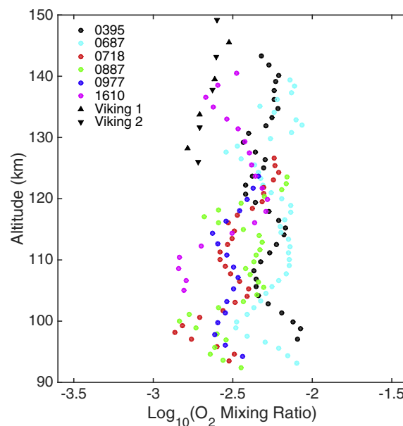
Fig. 15. The circles mark \text{O}_2 mixing ratios inferred from six UV stellar occultations ( Sandel et al., 2015 for orbits/ L_s of 0395/32.7°, 0687/68.9°, 0718/78.7°, 0887/93.5°, 0977/104.7°, 1610/195.4°). Error bars are omitted for clarity; typical values are in the range 10–25%. The numbers in the legend are the Mars Express orbit numbers. Geometry information about the sampled regions may be found in Table 2 . The triangles indicate values from the lower part of the altitude range sampled by Viking. These profiles suggest variations in \text{O}_2 mixing ratio in space and time.
