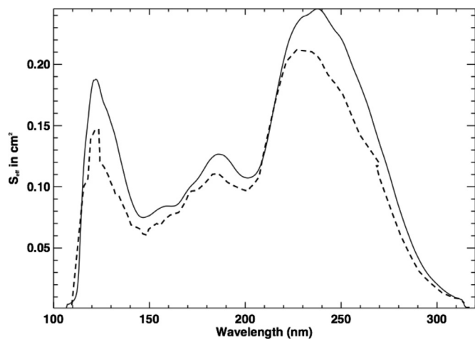
Fig. 3. Updated version of the efficient area Seff of the SPICAM UV channel based on the updated calibration procedure established by A. Reberac and reported in Snow et al. (2013). The previously published version of Seff (see Bertaux et al., 2006) is shown for comparison in dashed line.
