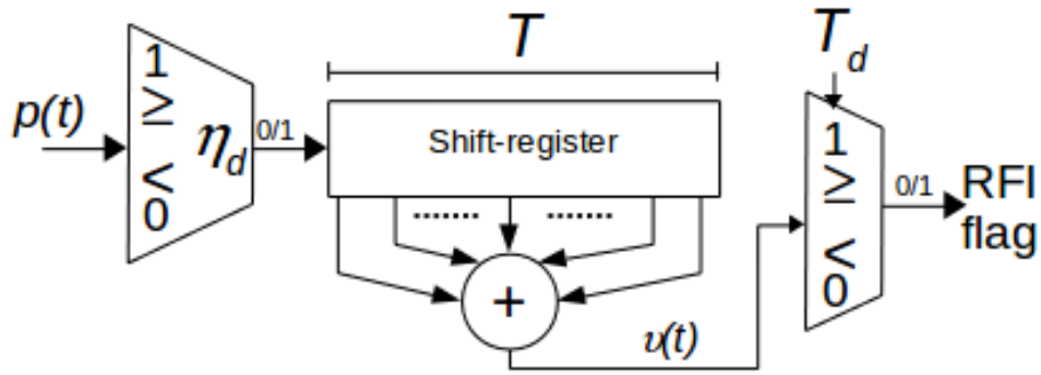
Fig. 6. Schematic view of the Bernoulli power detector. p(t) is the instantaneous power. \eta_d is the RFI power threshold. Depending on \hat{\sigma}_n^2(t) . The 1-bit shift-register is T samples long. The RFI flag is set to 1 when the number of 1 in the shift-register ( \nu(t) ) is greater or equal to T_d .
