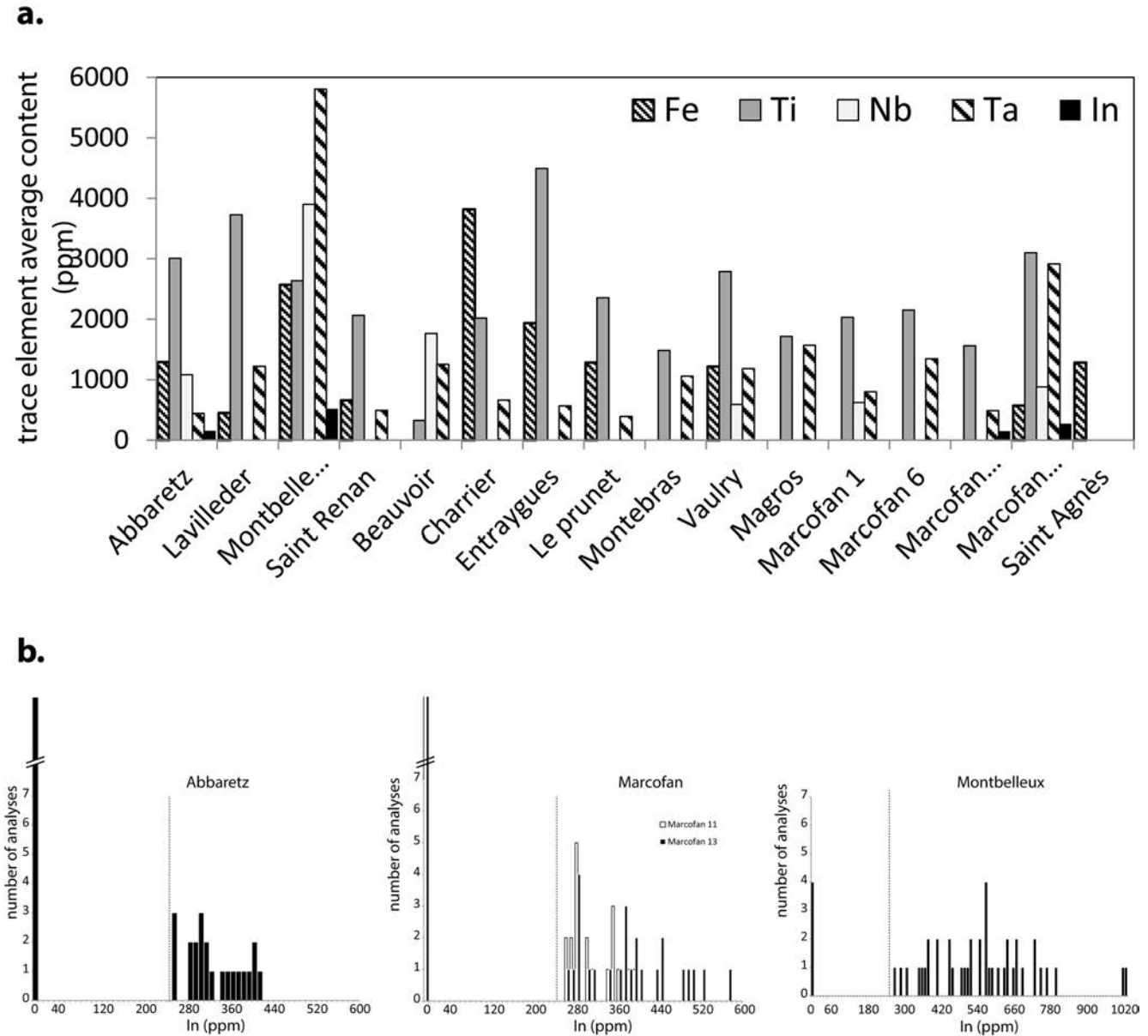
Fig. 2. (a) Histogram showing the average values of Fe, Ti, Nb, Ta and In contents in cassiterite from the thirteen Sn ore deposits; (b) histograms of indium grade distribution (ppm) for some cassiterite from Abbaretz, Marcofán and Montbelleux deposits. Bin size = 10 ppm, EPMA detection limit of 253 ppm is represented by the vertical dotted line on each histogram. The disrupted zero bins represent 78, 78 and 27 analyses for Abbaretz, Marcofán11 and Marcofán13, respectively.
