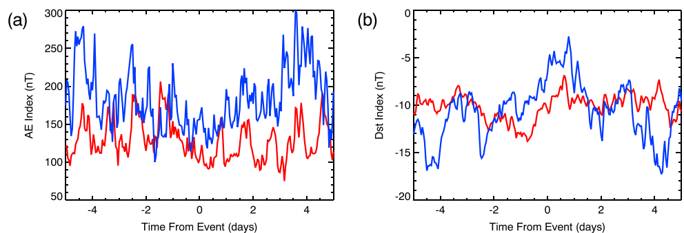
Figure 2. Superposed epoch analysis of the variation of geomagnetic indices around the times of all 87 TILR events. (a) Mean value of AE index as a function of the time relative to the times of the events. The results obtained for the events observed in the Northern Hemisphere are shown by the red curve, and the results obtained for the events observed in the Southern Hemisphere are shown by the blue curve. (b) The same as Figure 2a but for mean value of Dst index.
