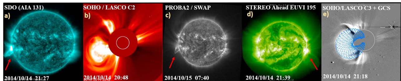
Figure 2. CME ejected on 14 October 2014 at ~18:30 UT. (a) SDO AIA image taken at 21:27 UT with 131 Å filter. (b) SOHO image from LASCO C2 taken at 20:48 UT. (c) PROBA-2 SWAP image taken at 07:40 UT on 15 October 2014. (d) STEREO-A SECCHI image at 21:39 UT using 195 Å filter. (e) GCS model fits to the LASCO C3 image. (f) (different temporal scale) PROBA-2/LYRA time series of solar radiation measured by the aluminum and zirconium filter channels. The red arrow in Figures 2a, 2c, and 2d indicates the CME source location. Note that STEREO-A is on the opposite side of the Sun from the Earth (Figure 1).
