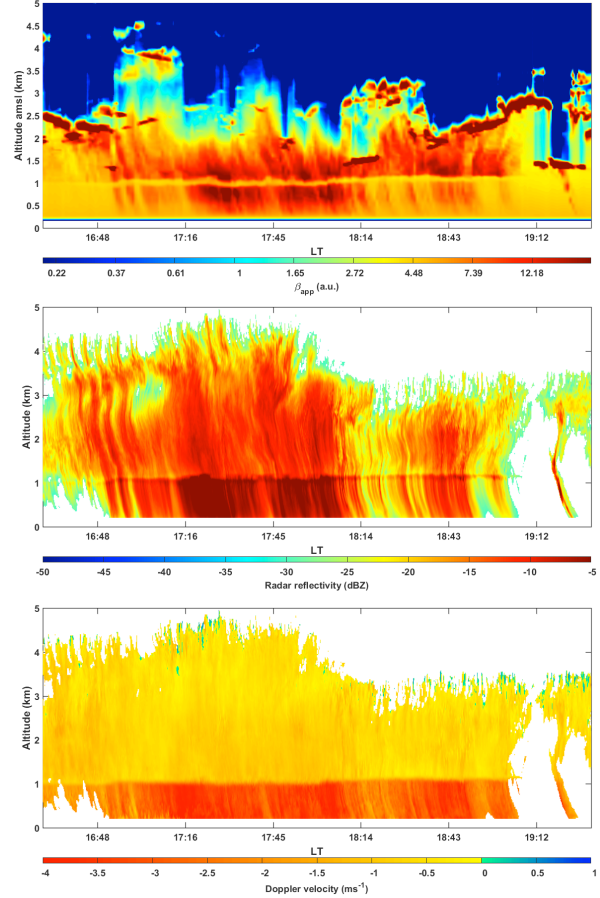
Figure 6. Temporal evolutions on 24 th May 2016 of the lidar-derived ABC_{app} (top panel), radar reflectivity in dBZ (middle panel), and Doppler radar-derived vertical drop speed (bottom panel).
