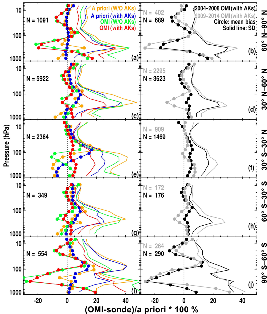
Figure 3. Mean relative biases in ozone (line with circles) and corresponding standard deviations (solid lines) between OMI retrieval–a priori and ozonesondes with and without (W/O) applying OMI retrieval averaging kernels (i.e., with AKs and without AKs in red and green for comparing retrievals and in blue and yellow for comparing a priori) for five different latitude bands. The left panels show the comparison using 10 years of OMI data (2004–2014), and the right panels show the comparison between OMI retrieval and ozonesonde with OMI AKs for before and after the occurrence of serious OMI row anomaly (RA), i.e., pre-RA (2004–2008) in black and post-RA (2009–2014) in gray. The number ( N ) of OMI–ozonesonde coincidences used in the comparison is indicated in the legends.
