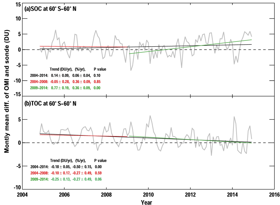
Figure 14. Same as Fig. 13 but for stratospheric ozone columns (SOCs) and tropospheric ozone columns (TOCs).
