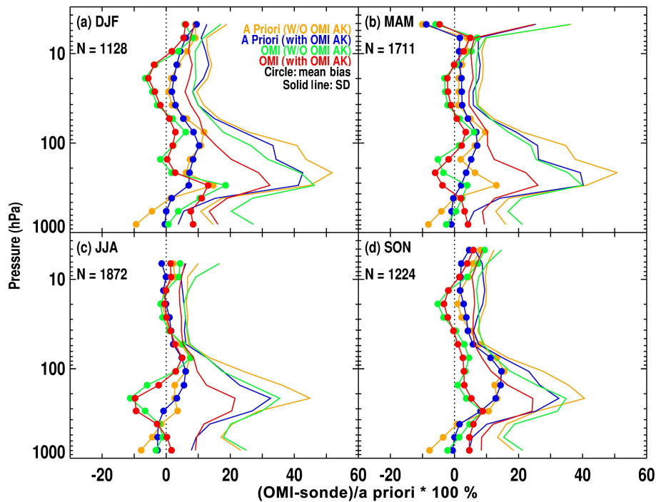
Figure 4. Same as Fig. 3c but for each individual season at 30–60° N.
