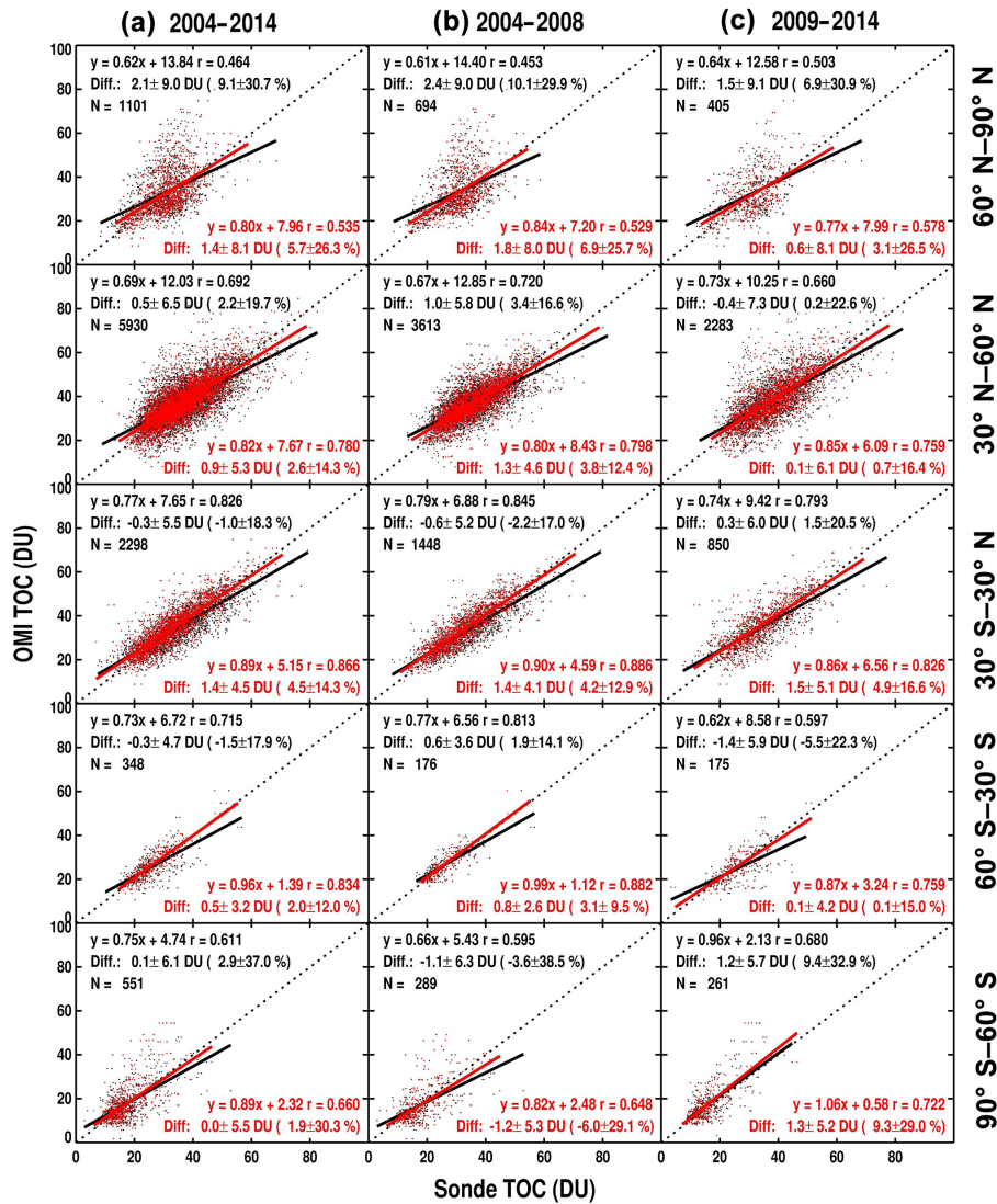
Figure 9. Similar to Fig. 8 but for comparison of tropospheric ozone columns (TOCs).
