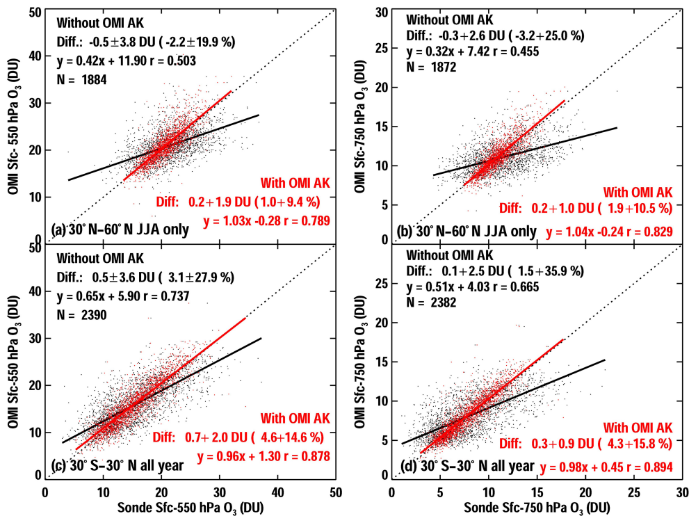
Figure 12. Similar to Fig. 9 but for comparison of lower tropospheric ozone columns during the 2004–2014 period. (a) Surface–550 hPa ozone column and (b) surface–750 hPa ozone column in 30–60° N during the summer; (c) and (d) same as (a) and (b) but for the tropics.
