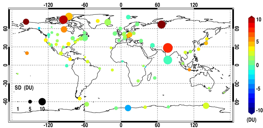
Figure 2. The distribution of ozonesonde stations in this study. The color represents the mean biases between OMI and ozonesonde tropospheric ozone columns (TOCs) at each station (if the number of OMI and ozonesonde pairs is more than 10), and the dot size represents the standard deviation.
