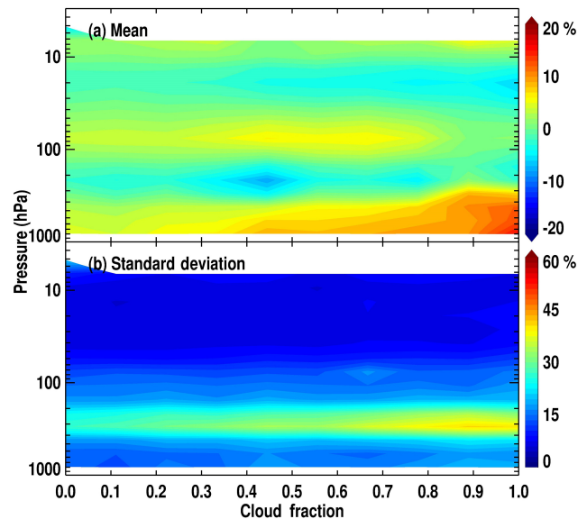
Figure 6. Same as Fig. 5 but as a function of cloud fraction.
