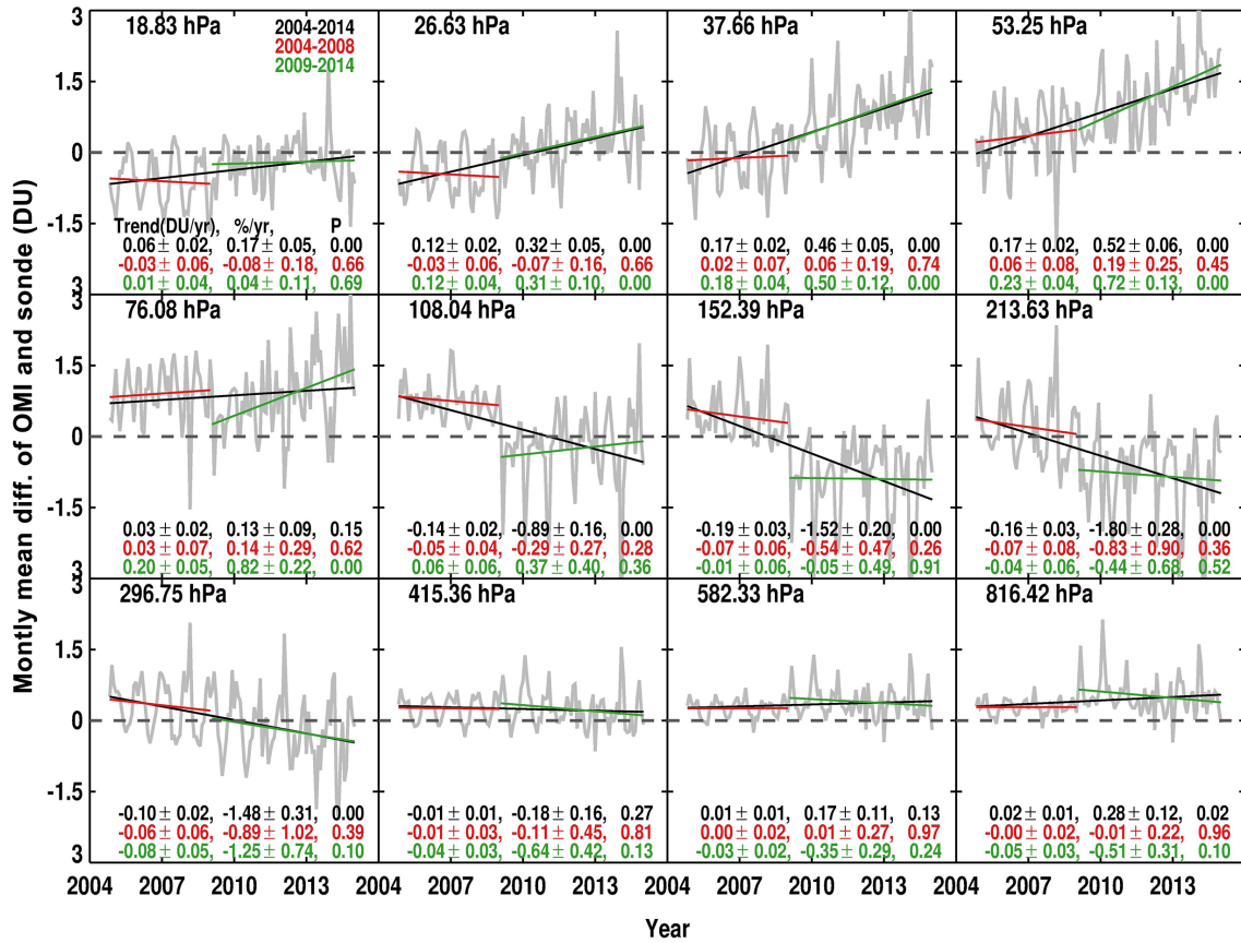
Figure 13. Monthly mean variation of OMI and ozonesonde mean biases in 60° N–60° S at each OMI layer. OMI retrieval averaging kernels are applied to ozonesonde data. The black, red, and green lines represent the linear ozone bias trends in 2004–2014, pre-RA (2004–2008), and post-RA (2009–2014), respectively. The average altitude of each layer is marked on the left corner of each grid. The trends in DU year -1 or % year and P value for each time period are indicated in the legends.
