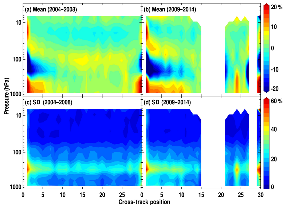
Figure 7. Same as Fig. 5 but as a function of cross-track position for (left) pre-RA (2004–2008) and (right) post-RA (2009–2014) periods.
