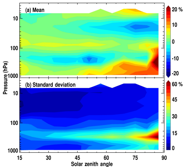
Figure 5. Mean relative biases in ozone (a) and standard deviations (b) of the differences between OMI and ozonesonde convolved with OMI AKs as a function of solar zenith angle using all OMI–ozonesonde coincidences during 2004–2014.
