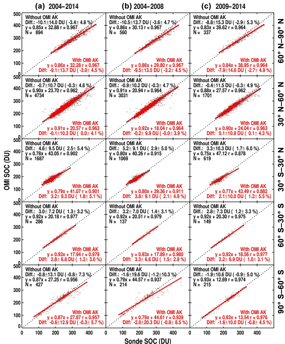
Figure 8. Scatter plots of OMI stratospheric ozone columns (SOCs) vs. ozonesonde SOC measurements without (black) and with (red) averaging kernels for five different latitude bands during 2004–2014 (a), the pre-row anomaly (RA) period (i.e., 2004–2008, b) and the post-RA period (i.e., 2009–2014, c), respectively. Comparison statistics including mean biases and standard deviations in both DU and %, the linear regression and correlation coefficients in DU, and the number of coincidences are shown in the legends.
