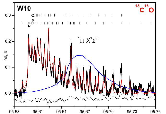
Fig. 5. ^{13}\text{C}^{18}\text{O} W(v=1) - X(0) band experimental absorption spectrum (black lines), and fit (red lines) and unknown band profile (blue). The fitting residuals are shifted by 0.04.
