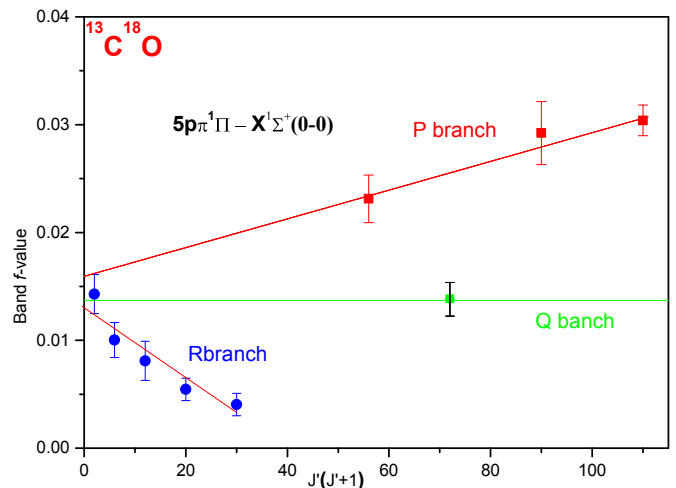
Fig. 15. ^{13}\text{C}^{18}\text{O} oscillator strength for the 5p\pi^1\Pi(v=0) - X(0) .
