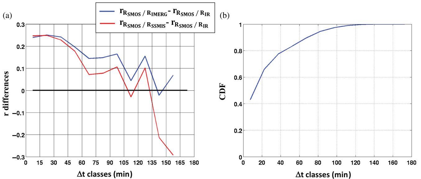
FIGURE 15 (a) Correlation between R_{\text{SMOS}} and R_{\text{IMERG}} minus correlation between R_{\text{SMOS}} and R_{\text{IR}} (blue line); correlation between R_{\text{SMOS}} and R_{\text{SSMIS}} minus correlation between R_{\text{SMOS}} and R_{\text{IR}} (red line), as function of temporal shift ( \Delta t ) between SMOS and nearest (in time) SSMIS. Size of \Delta t classes = 15 min. (b) CDF of number of pixels as function of temporal shift ( \Delta t ) between SMOS and nearest (in time) SSMIS
