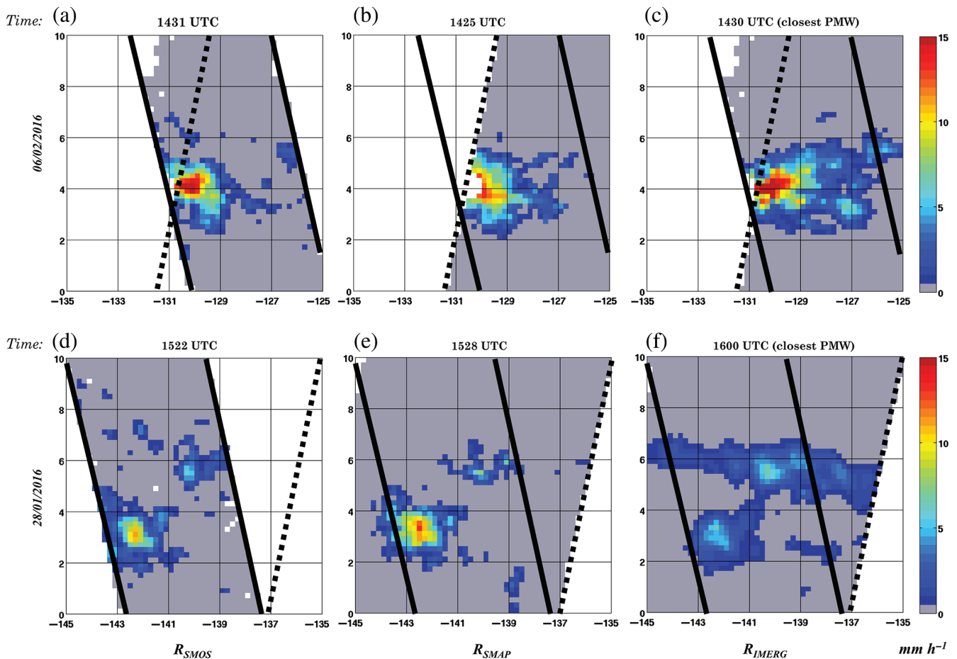
FIGURE 16 (a–c) Case-study of 6 February 2016, short temporal shift between SMOS/SMAP and the closest PMW: (a) R_{\text{SMOS}} ; (b) R_{\text{SMAP}} ; (c) R_{\text{IMERG}} . (d–f) Case-study of 28 January 2016, long temporal shift between SMOS/SMAP and the closest PMW: (d) R_{\text{SMOS}} ; (e) R_{\text{SMAP}} ; (f) R_{\text{IMERG}} .
