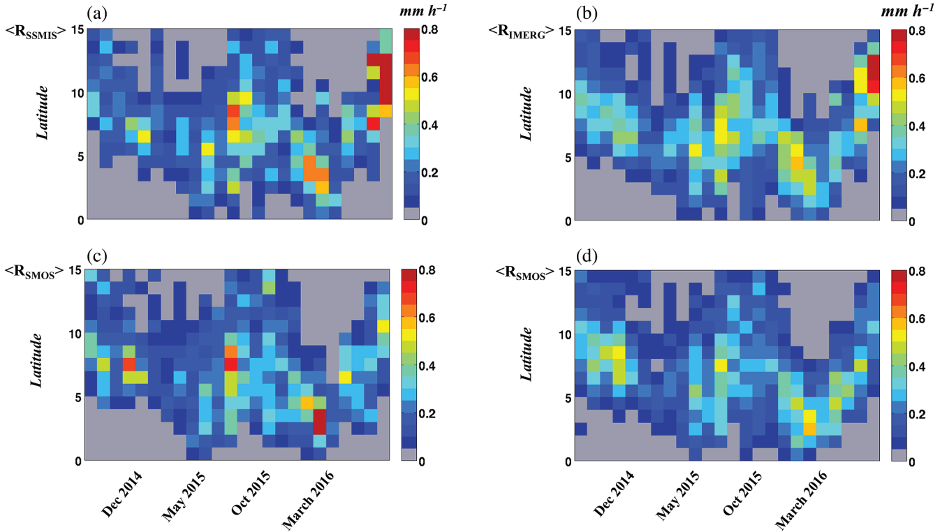
FIGURE 12 (a, c) SSMIS collocated with SMOS in 15 min time interval with (a) Hovmöller diagrams of R_{SSMIS} and (c) Hovmöller diagrams of R_{SMOS} ; (b, d) IMERG collocated with SMOS (but only with SSMIS as nearest collocated rain satellite) with (b) Hovmöller diagrams of R_{IMERG} and (d) Hovmöller diagrams of R_{SMOS} . With an orthogonal regression \langle R_{SMOS} \rangle = 1.03 \langle R_{SSMIS} \rangle + 0.00 ( r = 0.89 ; RMSD = 0.07 ) and \langle R_{SMOS} \rangle = 0.90 \langle R_{IMERG} \rangle + 0.01 ( r = 0.92 ; RMSD = 0.06 ) after exclusion of pixels above 9^\circ N during the last 2 months of the study period
