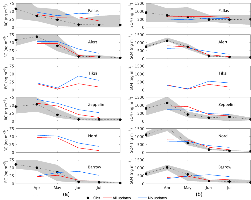
Figure 7. Monthly median BC (left) and \text{SO}_4^{2-} (right) observations at Arctic surface stations (gray shading indicates 25th and 75th percentile) and corresponding WRF-Chem results (red, ALL_UPDATES; blue, NO_UPDATES).
