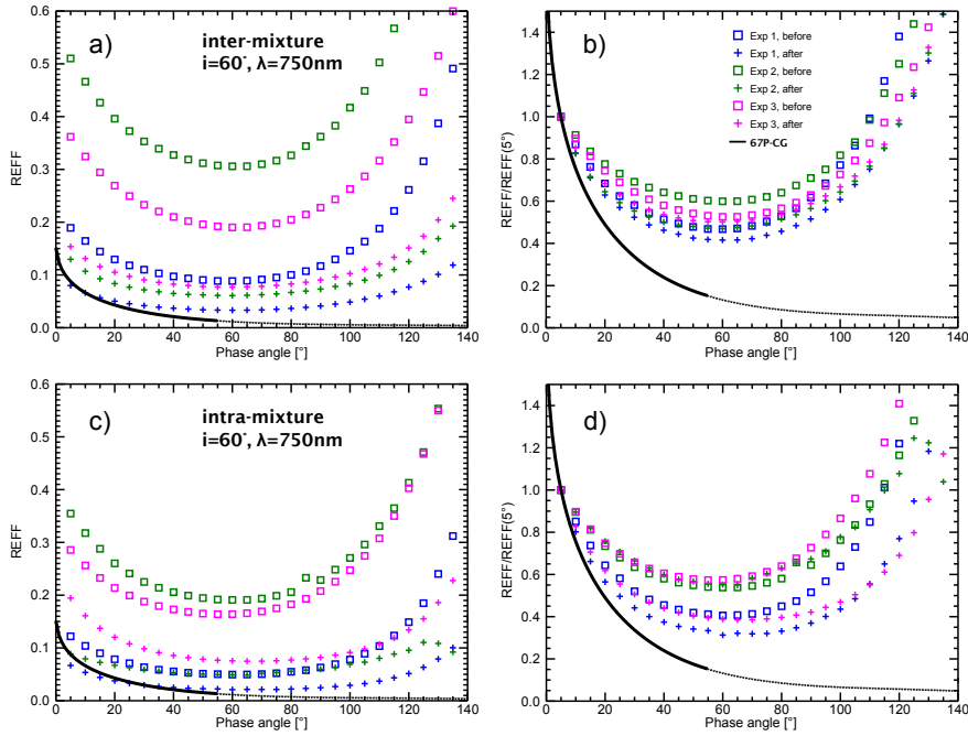
Figure 12: Phase curves of all experiments measured at i = 60^\circ and \lambda = 750\text{nm} before and after sublimation. a) Inter-mixtures in absolute reflectance, b) normalized at \alpha = 5^\circ , c) intra-mixtures in absolute reflectance, d) normalized at \alpha = 5^\circ . All samples decrease in reflectance after sublimation in thermal vacuum and become less scattering in the forward direction. The intra-mixtures display a higher variation in shape when normalized than the inter-mixtures. After sublimation the intra-mixtures have lower reflectances at high phase angles, which is consistent with a higher surface roughness or porosity.
