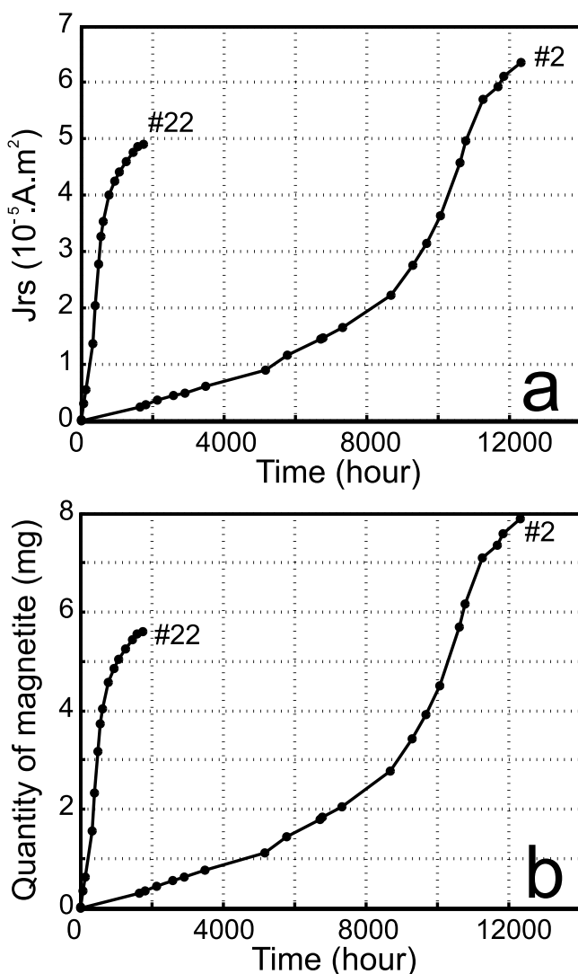
Figure 6. (a) J_{rs} as a function of time for Run 22 and Run 2 (300°C/500 bars) with an initial olivine grain size of 5–15 \mu\text{m} and 50–63 \mu\text{m} , respectively. (b) Same as Figure 6a but plotting the derivation of the amount of magnetite produced using J_{rs}/J_s measurements.
