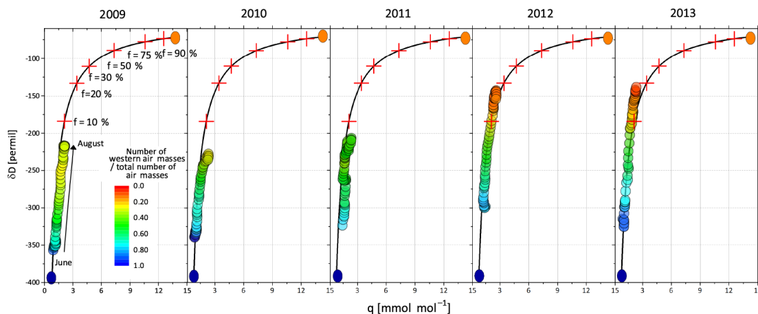
Figure 10. Summer enrichments (from June to August) observed at the CAR from 2009 to 2013 along a mixing model defined by the mixing between upper tropospheric water vapour (UT) and boundary layer vapour above the Mediterranean (MBL). IASI daily observations at 5.5 km are smoothed on a 30-day moving average filter and the corresponding ratios of western air masses to total number of air masses are shown in colour. The 10, 50, 75, and 90% fractions ( f ) of MBL of Eqs. (2) and (3) are indicated with the red crosses.
