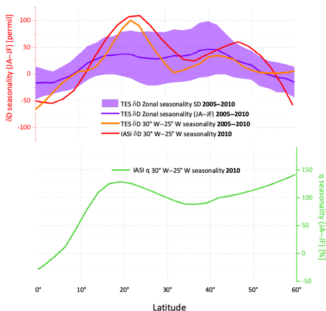
Figure 7. Top panel: global \delta\text{D} zonal seasonality (JA–JF) from 0 to 60° N (purple line) with its associated standard deviation (shaded area) and seasonality found offshore of West Africa (30–25° W, 0–60° N) (orange line) observed by TES for the 2005–2010 period and as observed by IASI seasonality for 2010 (red line). Bottom panel: IASI specific humidity seasonality.
