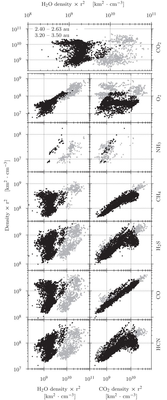
Figure 7. Top: scatter plot of CO 2 versus H 2 O. Lower left graphs: scatter plots of the studied species versus H 2 O. Lower right graphs: scatter plots of the studied species versus CO 2 . The measurements shown here belong to the time period 2016 February 19–2016 March 23 (2.40–2.63 au, grey), and June 13–August 1 (3.20–3.50 au, black).
