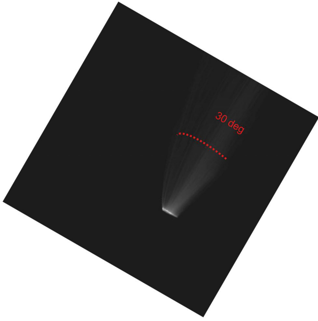
(a) Trajectories of the dust (radius 1.97 \mu\text{m} )
