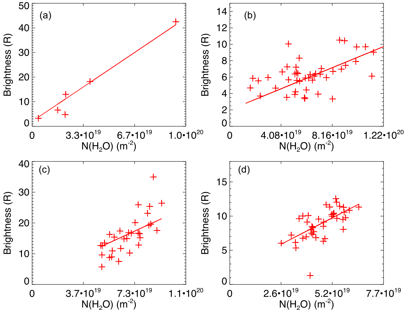
Figure 6. Lyman \beta brightness measured by Alice versus the water vapour column density measured by VIRTIS-H on 2014 December 3–9 (a), 2015 March 12 and 13 (b), 2015 May 13 and 14 (c) and 2015 May 25–26 (d). The best linear fits are represented by the red lines.
