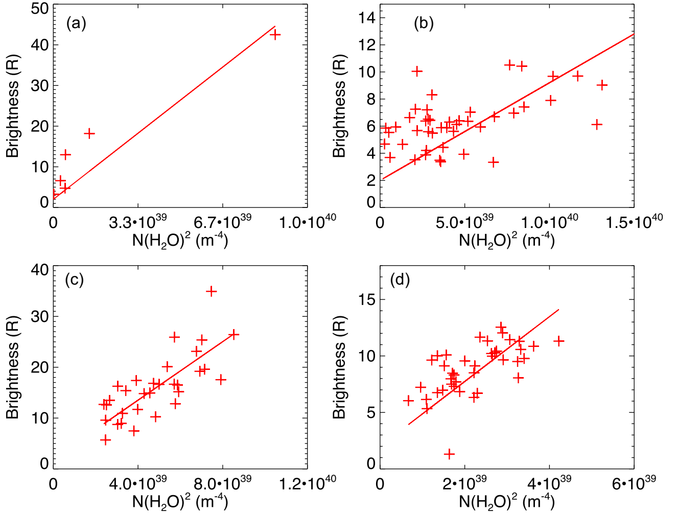
Figure 5. Lyman \beta brightness measured by Alice versus the square of the water vapour column density measured by VIRTIS-H on 2014 December 3–9 (a), 2015 March 12 and 13 (b), 2015 May 13 and 14 (c) and 2015 May 25–26 (d). The best linear fits are represented by the red lines.
