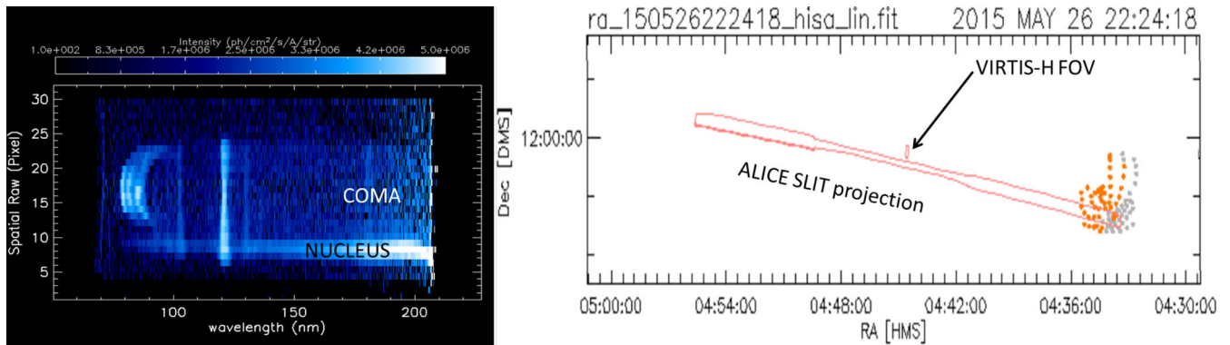
Figure 1. Left: Image of the detector of Alice observed during one observation on 2015 May 26. Right: The geometry of the observation and the sky projection of the Alice slit and VIRTIS field of view are indicated in red. The small VIRTIS field of view is indicated by the arrow. The right figure is derived from geoviz tool using the SPICE digital Shape Kernel (DSK) for the comet. Orange dots indicate the sunlit face of the comet and the grey dot the unlit portion of the comet.
