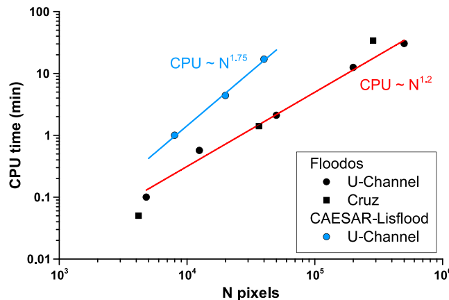
Figure 13. Computation time as a function of the number of wet pixels (Table 1) for the U -shaped channel (solid black circles) and Cruz case (solid black squares). For the U -shaped channel (see section 3.2), the computation time was recorded in the stationary regime. Calculations were performed using the largest time step value that respected the stability criteria defined in section 3.2. The computation time increased slightly nonlinearly with the number of pixels following a relationship: CPU time \sim N^{1.2} . The computation time followed a similar pattern for the real-case application ("Cruz," black square) described in section 3.4. For comparison, the results obtained with Lisflood-FP are indicated (blue dots). Although all the simulations are performed on the same computer, this test cannot be considered as a benchmark of both codes since Lisflood-FP calculates the transient regime, and it can certainly be better optimized if run by its developers.
