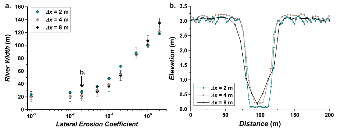
Figure 9. (a) River width at stationary stage for three different grid resolutions ( \Delta x = 2, 4, 8 m) as a function of the lateral erosion parameter k_e defined in equation (17). (b) Channel cross section at the model center for k_e = 2.10^{-2} . All the other simulation parameters are described in the text.
