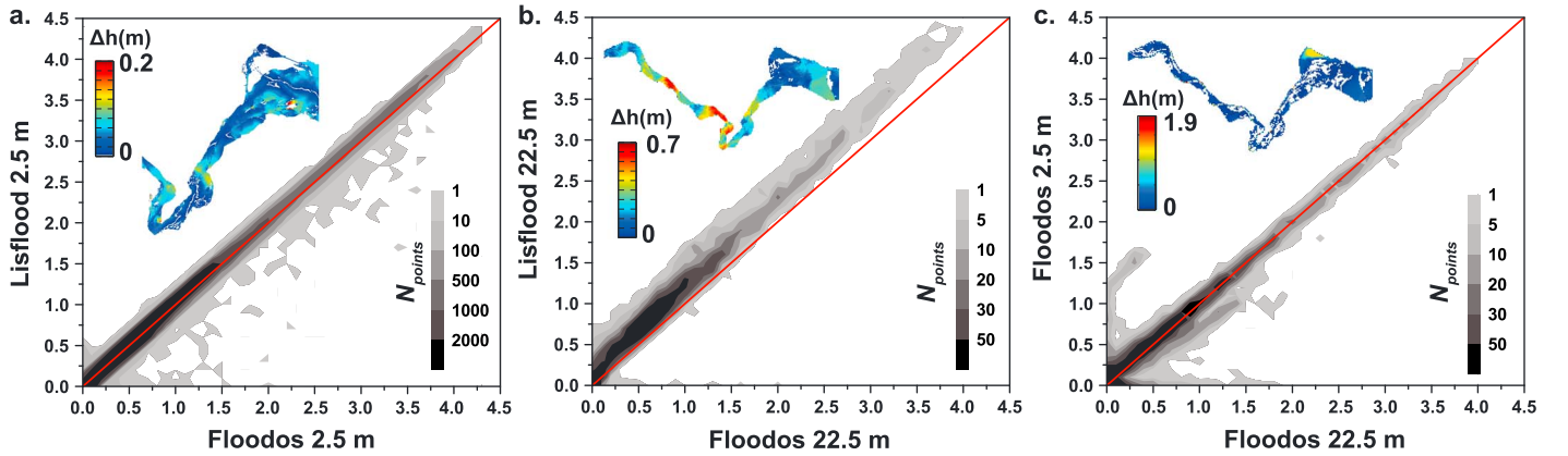
Figure 7. Density plot of the comparisons between Floodos and Lisflood-FP water depth predictions for different grid resolutions (red line is h_{\text{Floodos}} = h_{\text{Lisflood}} ) along with a raster map of the difference of water depth predictions (a) \Delta x = 2.5 m and (b) \Delta x = 22.5 m. (c) Density plot comparing Floodos water depth predictions for the same DEM with two resolutions of 2.5 m and 22.5 m, respectively.
