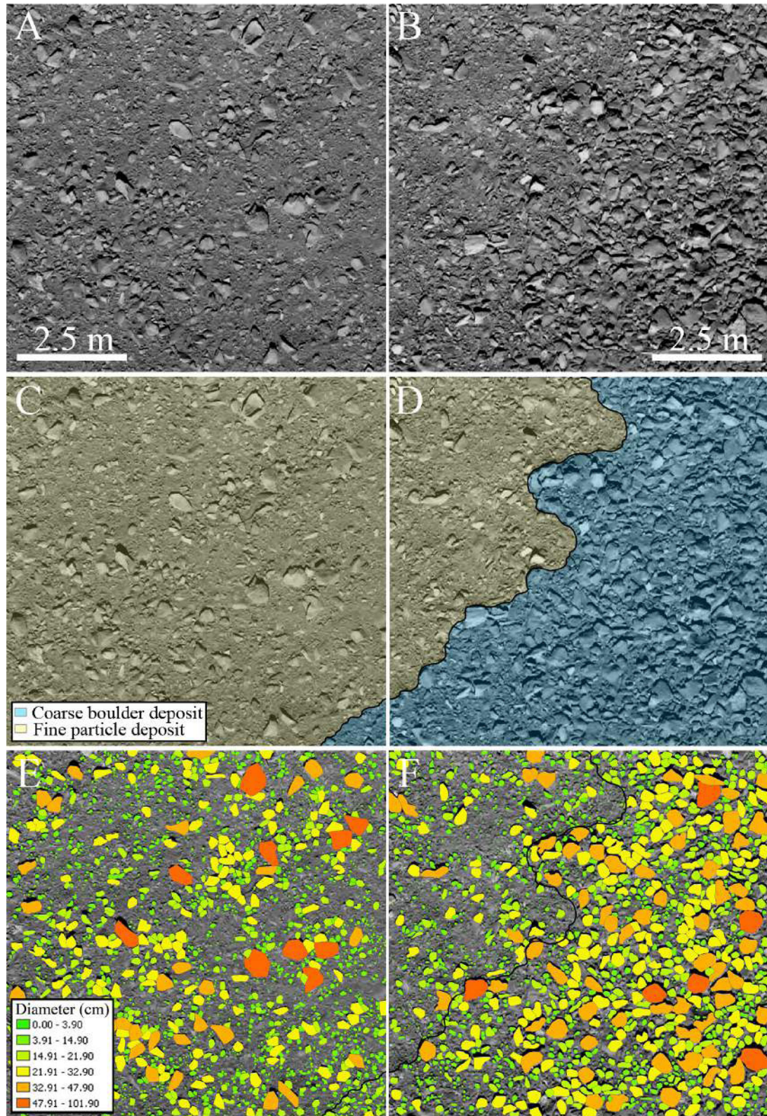
Figure 4. (A): WAC image taken on 2016 September 30 at 10:36:55 UT 138 m from the nucleus surface. (B): WAC image taken on 2016 September 30 at 10:37:04 UT 130 m from the nucleus surface. (C) and (D): morphological maps showing the two pebbles/boulders textures on Sais. (E) and (F): the spatial distribution of the pebbles/boulders identified on the WAC images. The pebbles/boulders are classified on their different sizes. (For interpretation of the references to colour in this figure legend, the reader is referred to the web version of this article.)
