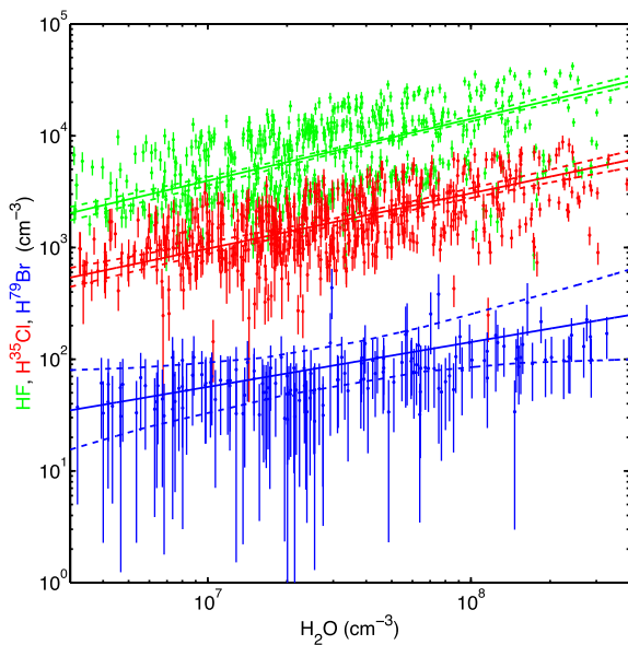
Figure 5. Hydrogen halide abundances relative to water. While the hydrogen halide densities vary with that of water, they are not linearly proportional. The error margins reflect the Poisson uncertainties. Uncertainties on the sensitivities would systematically shift the curves somewhat, without altering their slope. Additional uncertainty due to the interpolation of the measurements to a common time-scale has not been included in the error bars, but such errors are limited as care has been taken to use hydrogen halide and water abundances acquired with minimal time delay. The measurements are from period A (2014 October 1–24).
