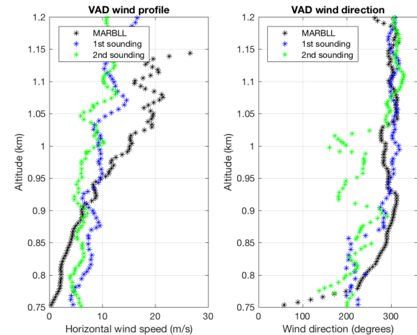
Figure 4: Profiles of wind speed (left) and direction (right) extracted from the VAD analysis and two radio soundings (1 st in the beginning of the MARBLL sequence, 2 nd 30 minutes after the end of the sequence). MARBLL errors increase significantly above 0.95 km.
