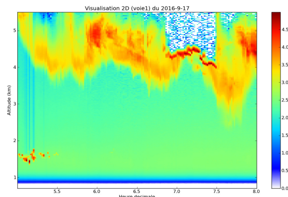
Figure 6: ICOS lidar range-corrected signal (arbitrary units) @ 532 nm vs. altitude from 5 to 8 UT.
