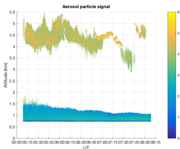
Figure 5: MARBLL range corrected signal @ 1064 nm (arbitrary units, SNR > 10) as a function of altitude from 5 UT to 8 UT (sunrise at 5:20 UT).
