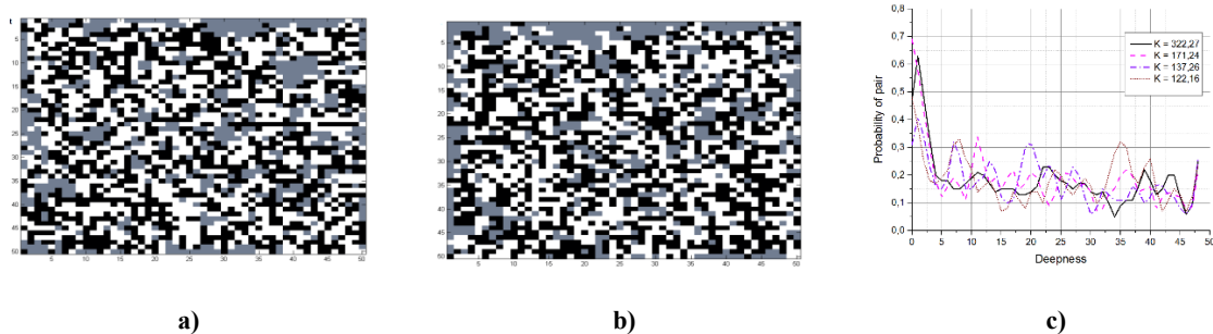
Figure 5: 2D distribution with 4 free edges (RS): Topology a) and b) and c) Probability of pairs for different values of K (eV)
