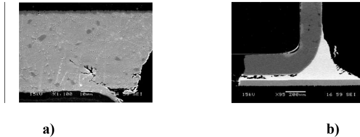
Figure 1: a) Cracks and voids after thermal shocks test 1h/1h a) ASIC (683 cycles, -40/+105°C) b) Melf Resistor (1000 cycles, -40/+125°C)
