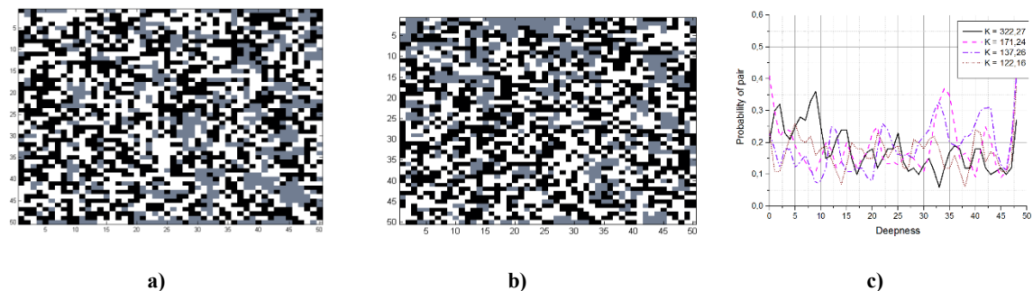
Figure 6: 2D distribution with 1 free edge (RS): Topology a) and b) and c) Probability of pairs for different values of K (eV)
