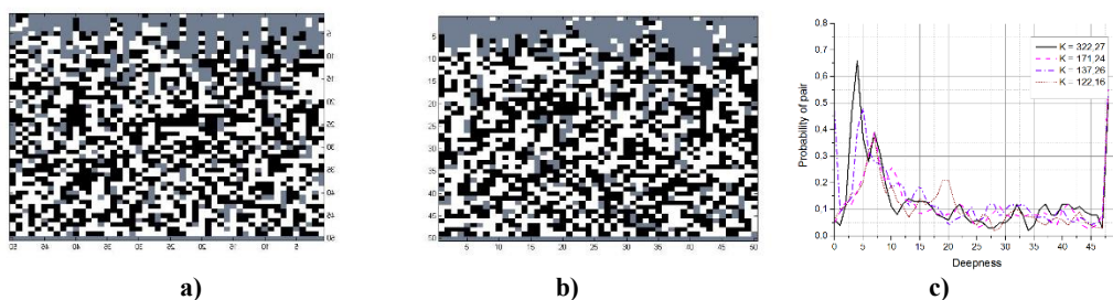
Figure 4: 2D distribution with 1 free edge (CS): Topology a) and b) and c) Probability of pairs for different values of K (eV)
