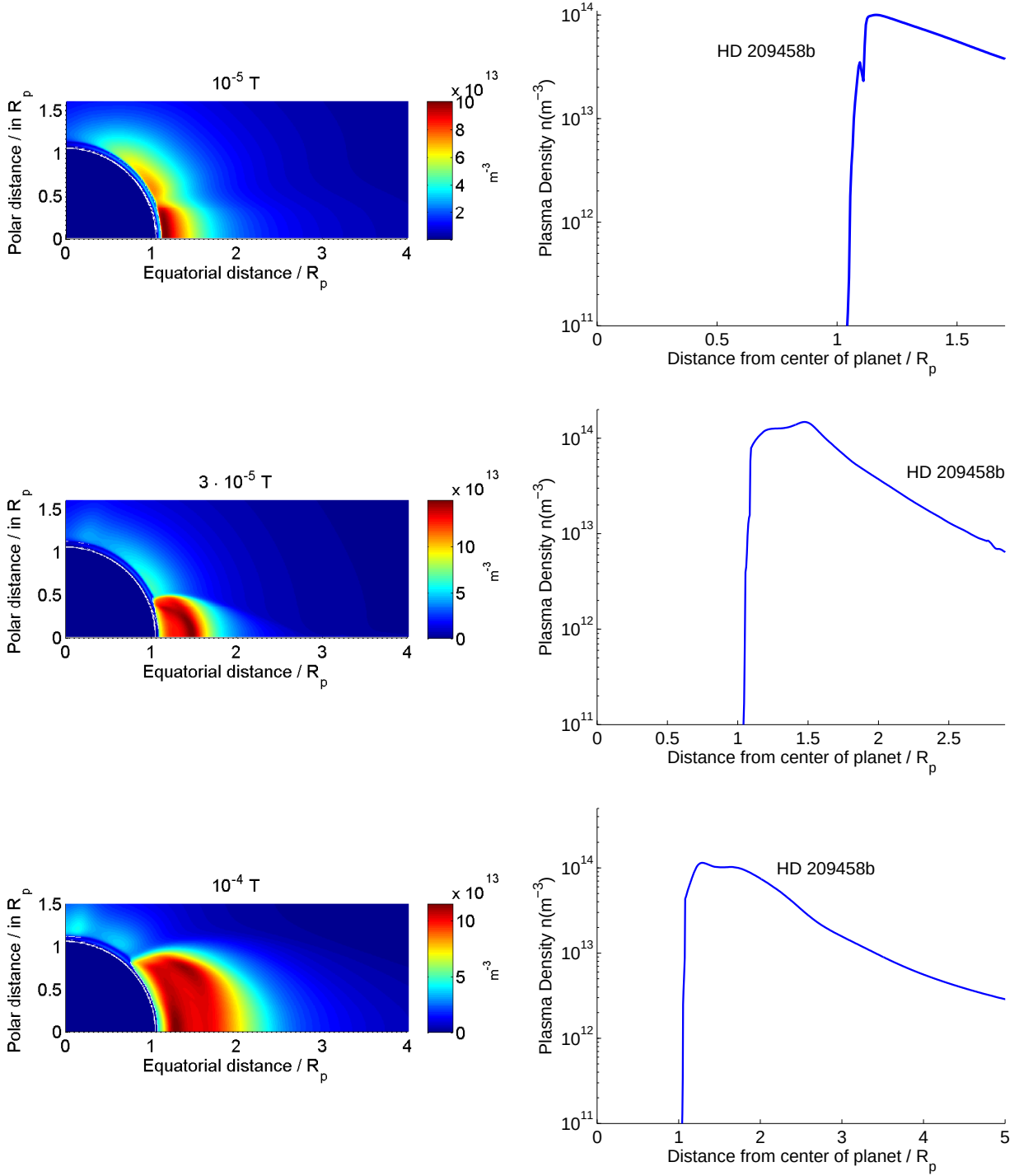
Figure 2. Plasma density in m^{-3} for HD 209458b (Shaikhislamov et al. 2014; Khodachenko et al. 2015) for the three values of equatorial surface magnetic field. Axes are scaled in planetary radii. The star is located to the right. The plots on the left-hand side are cross sections in the plane spanned by the line connecting the star and the planet (along the equator) and the polar axis. The figures on the right-hand side show corresponding density profiles along the equator towards the star. The profile curves end at the magnetopause. The magnetosphere is filled up with dense plasma up to the magnetopause, a case completely different from and not comparable to Earth or Jupiter.
