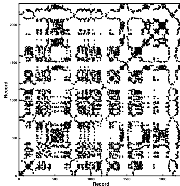
Figure 5. The RP for the HILDCAA example. The interval shown by the vertical dotted lines in Fig. 1 is used to obtain the plot.
