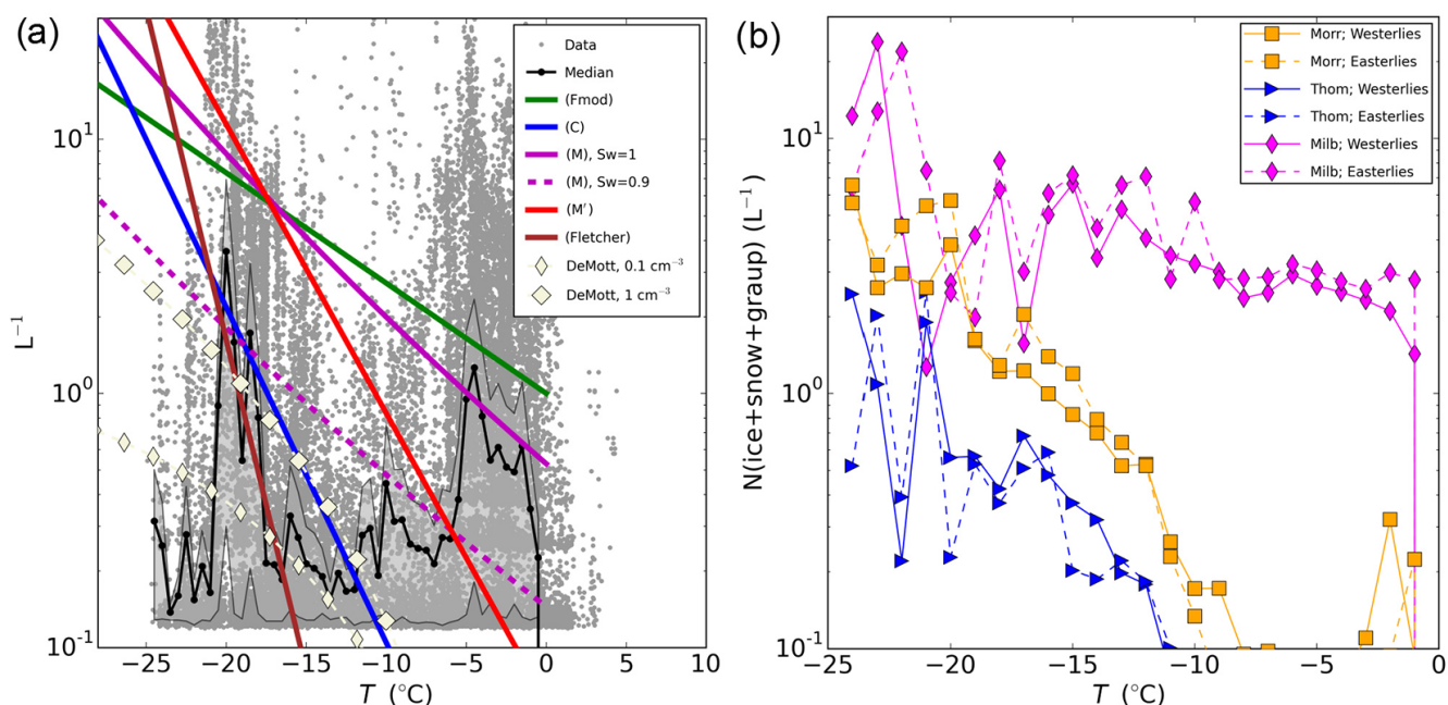
Figure 13. (a) Ice crystal measurement data points as a function of the temperature (grey) with their median per 0.5^{\circ}C bins (black solid line), along with the absolute median deviation in shaded grey. The labelled INP parameterizations used by the different cloud schemes (Table 3) are overlaid. DeMott refers to the DeMott et al. (2010) INP parameterization (see text for details). (b) Same as panel (a) but for the median of the total number concentrations of icy hydrometeors in the same transects used in Fig. 5 for both cases: the westerly case (solid lines) and the easterly case (dashed lines).
