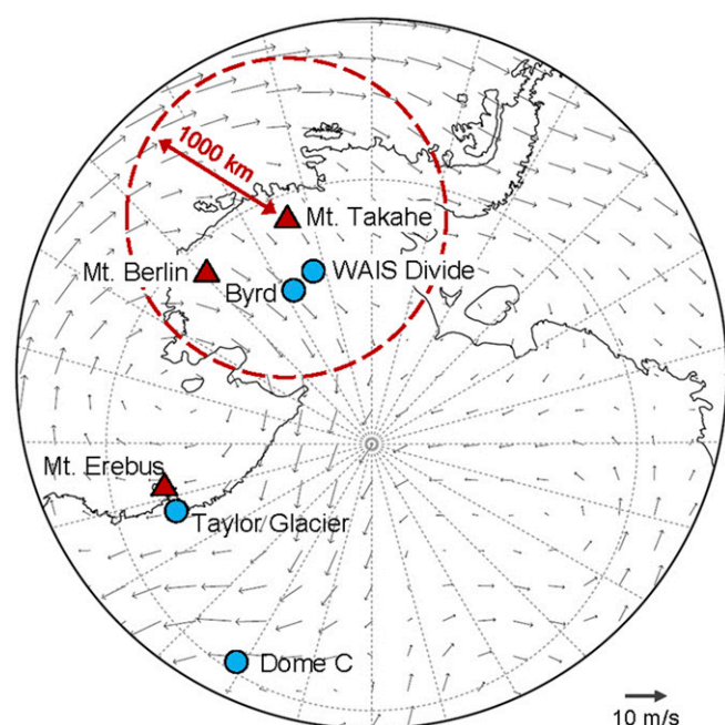
Fig. 3. Spatial extent of the glaciochemical anomaly. Evidence of the ~192-y anomaly has been found >2,800 km from Mount Takahe in ice core (circles) chemical records ( SI Appendix, Fig. S3 ) as well as radar surveys from much of West Antarctica. Also shown are area volcanoes (triangles). September/October horizontal wind vectors at 600 hPa based on 1981–2010 National Centers for Environmental Prediction reanalysis fields show transport patterns consistent with observations.
