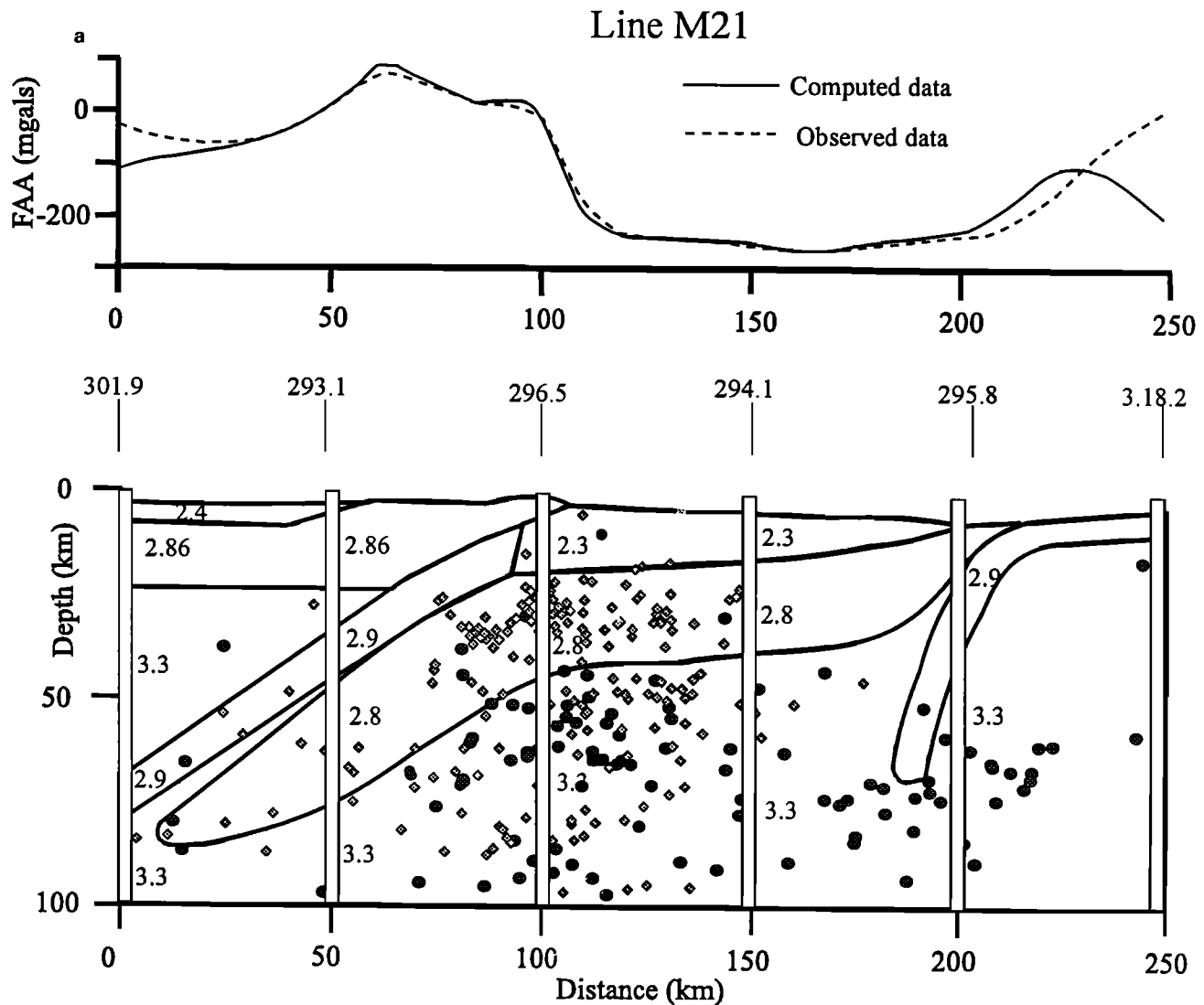
Figure 9. Two-dimensional gravity modeling for (a) line M21 and (b) line M31 (locations in Figure 1 and 4). Digits inside the polygons are the chosen densities. Observe the rupture of the crust beneath the accretionary wedge and the underplating of the Snellius Ridge beneath the long west dipping Molucca slab. Diamonds indicate the seismicity recorded by the OBS network during the MODEC cruise. Circles indicate the global seismicity. Mass columns are in \text{kg}/\text{cm}^2 .
