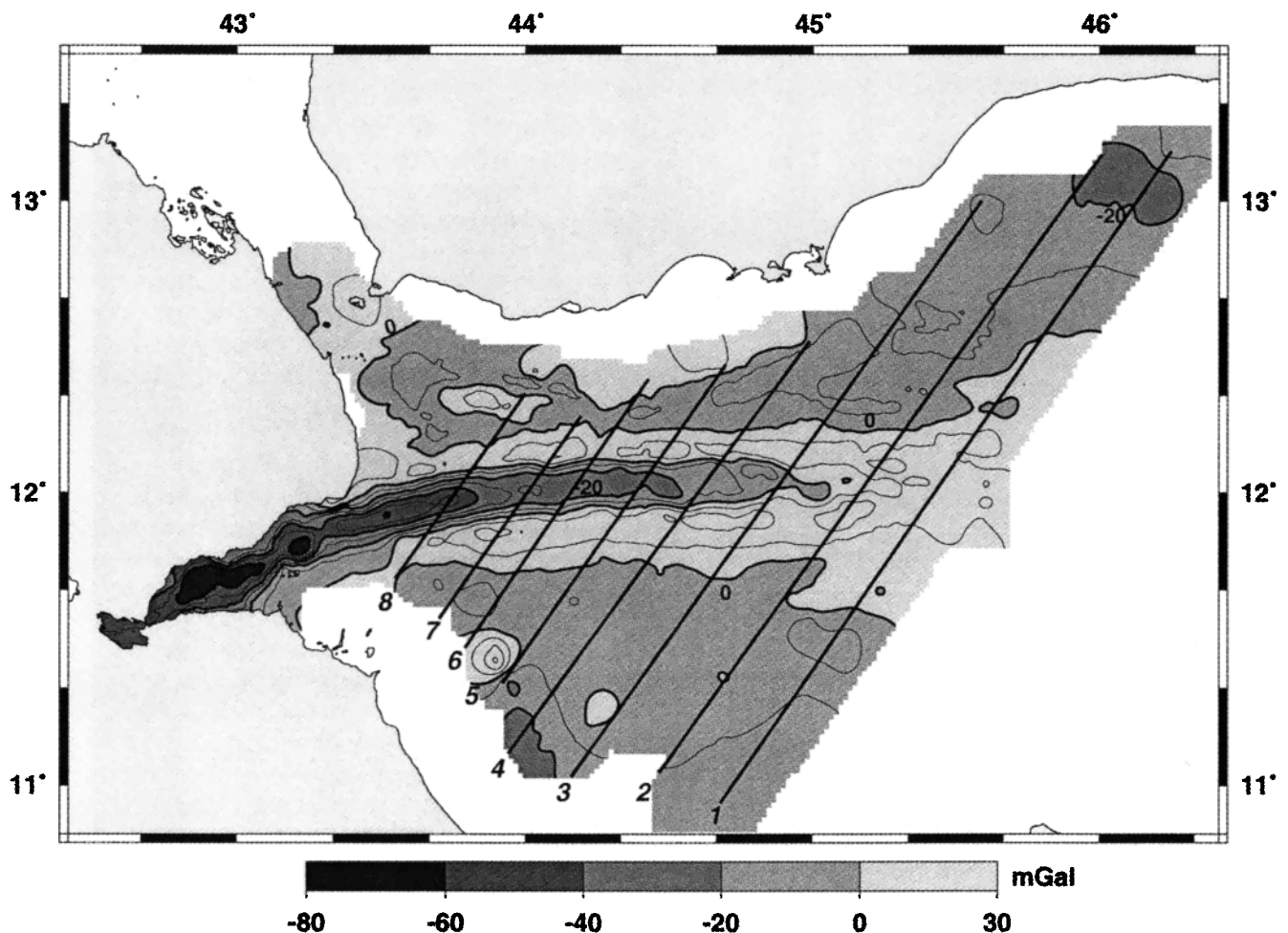
Figure 4. Free air anomaly computed from the Bodensewerk gravity data merged with the GPS navigation. For drawing purposes the gravity values gathered along tracks have been sampled on a 1 km grid using the adjustable tension surface gridding algorithm from the Generic Mapping Tools (GMT) software. Contours at 10 mGal intervals are shown, with thicker contours at 20 mGal intervals. Numbered lines indicate the locations of the profiles displayed in Figure 5.
