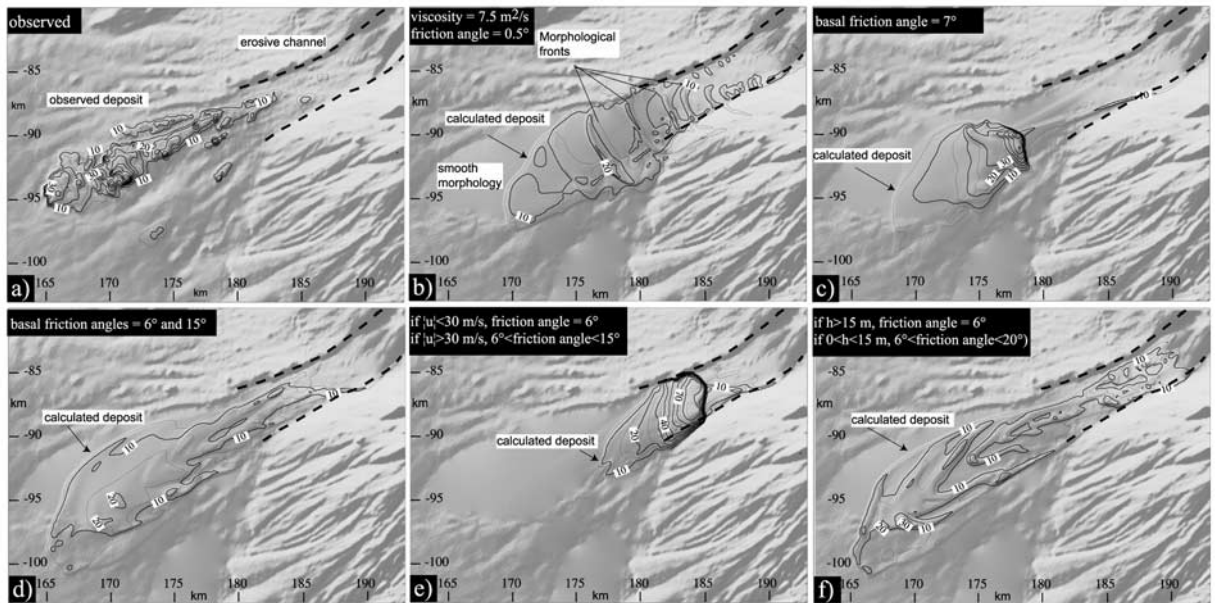
Figure 2. a) Observed deposit thickness superimposed on shaded bathymetry. Contour interval is 5 m. 10 m contour lines are annotated. 2b–f) Calculated deposit thickness superimposed on shaded bathymetry (pre-failure bathymetry + calculated deposit) : b) Viscous-Coulomb friction's model, c) Coulomb-type friction's law, d) Pouliquen's law, e) Coulomb-type friction's law with variable friction angle as a function of velocity, f) Coulomb-type friction's law with variable friction angle as a function of thickness.
