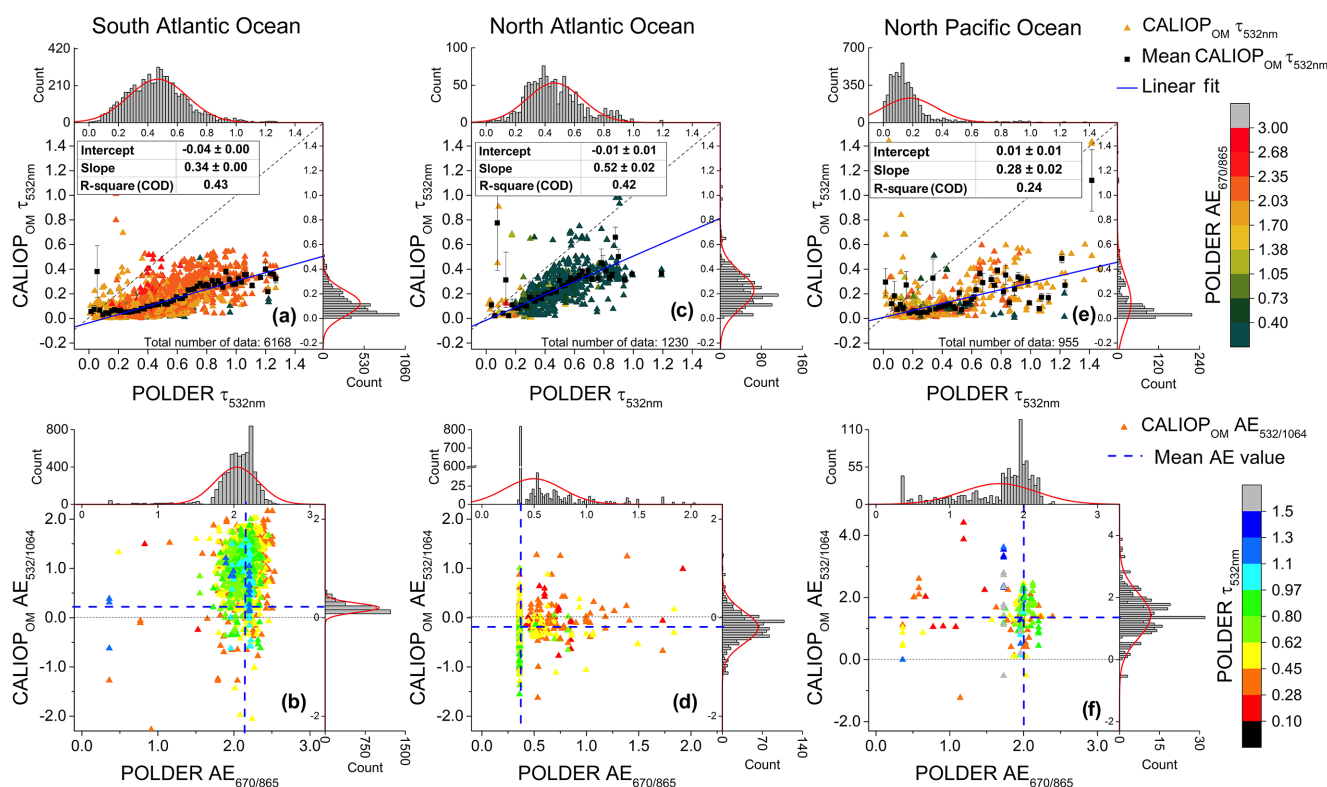
Figure 4. Same as Fig. 3, retrieved from CALIOP operational method and POLDER method.
