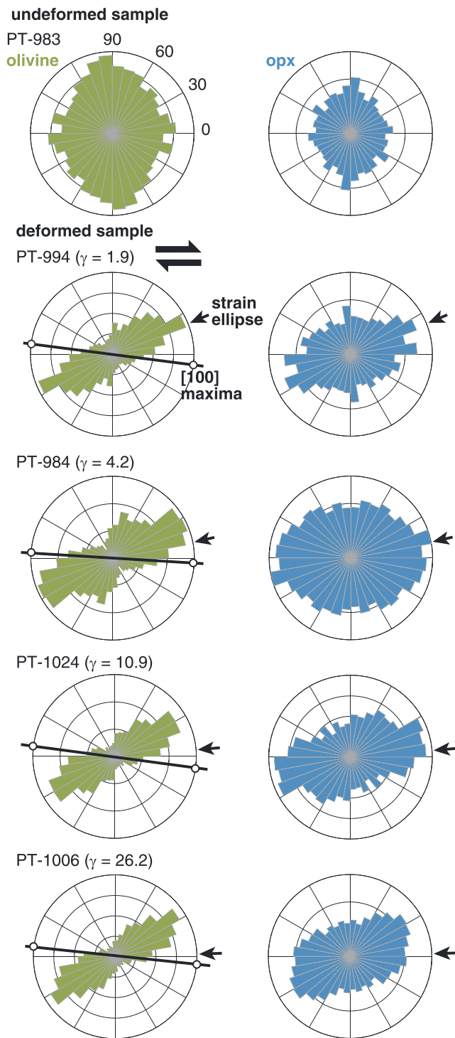
Figure 4. Rose diagrams illustrating the SPOs of olivine and pyroxene grains for the undeformed sample and for samples deformed at a strain rate of \sim 2 \times 10^{-4} \text{ s}^{-1} . The thick black line with open circles for the deformed samples indicates the olivine [100] CPO maxima from Figure 8. The angle between the SPO and CPO lines in the range 30 to 40° regardless of shear strain. The contour lines for frequency in the rose diagram are drawn every 50 grains. The angle of the strain ellipse long axis calculated from the measured shear strain is illustrated by a black arrow. The same texture analysis data were used to determine grain size distribution in Figure 3.
