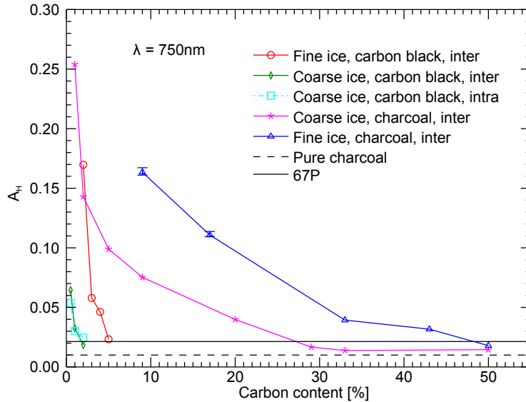
Figure 5: Hemispherical albedo of ice-carbon mixtures as function of carbon content all measured at i = 0^\circ and \lambda = 750\text{ nm} . Albedos of pure charcoal and 67P are plotted as horizontal reference lines. All possible combinations of ice grains (fine/coarse) and carbon particles (charcoal/carbon black) are shown. Further the combination of coarse ice particles and carbon black was produced using both mixing types (inter/intra mixture), but resulted without noticeable difference in albedo. Generally spoken it can be stated that mixtures of fine grained ice are brighter than with coarse grains when using the same carbon content. Vice versa smaller carbon particles have a bigger darkening effect than bigger ones, when using the mixing ratios. Both findings can be explained by changing total surface area per mass.
