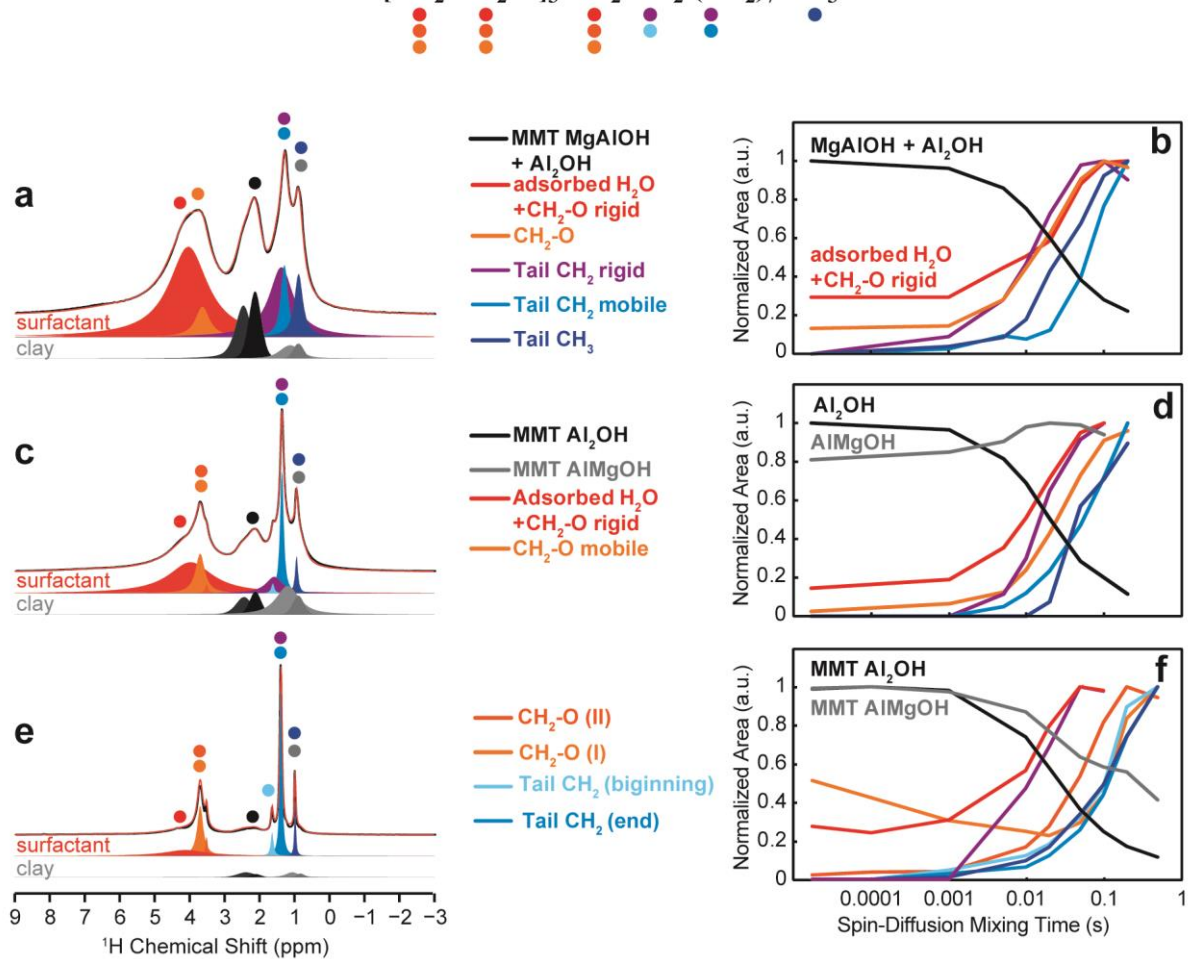
Figure 8. (a,c,e) Quantitative ^1\text{H} NMR spectra (in black) with the corresponding model (in red) and individual components (same color code as in Fig. 8) for Mt- \text{C}_{10}\text{E}_3 organoclay samples # (a) 1, (c) 2, and (e) 3 prepared with initial surfactant concentrations of 5 \times 10^{-4} , 2 \times 10^{-3} , and 7.5 \times 10^{-3} mol.L ^{-1} , respectively. (b,d,f) Normalized intensities measured for all individual components using the experiment described in Figure 8, and plotted as functions of the ^1\text{H} - ^1\text{H} spin-diffusion mixing time during which the ^1\text{H} magnetization diffuses from clay hydroxyl sites to the surfactant ^1\text{H} nuclei.
