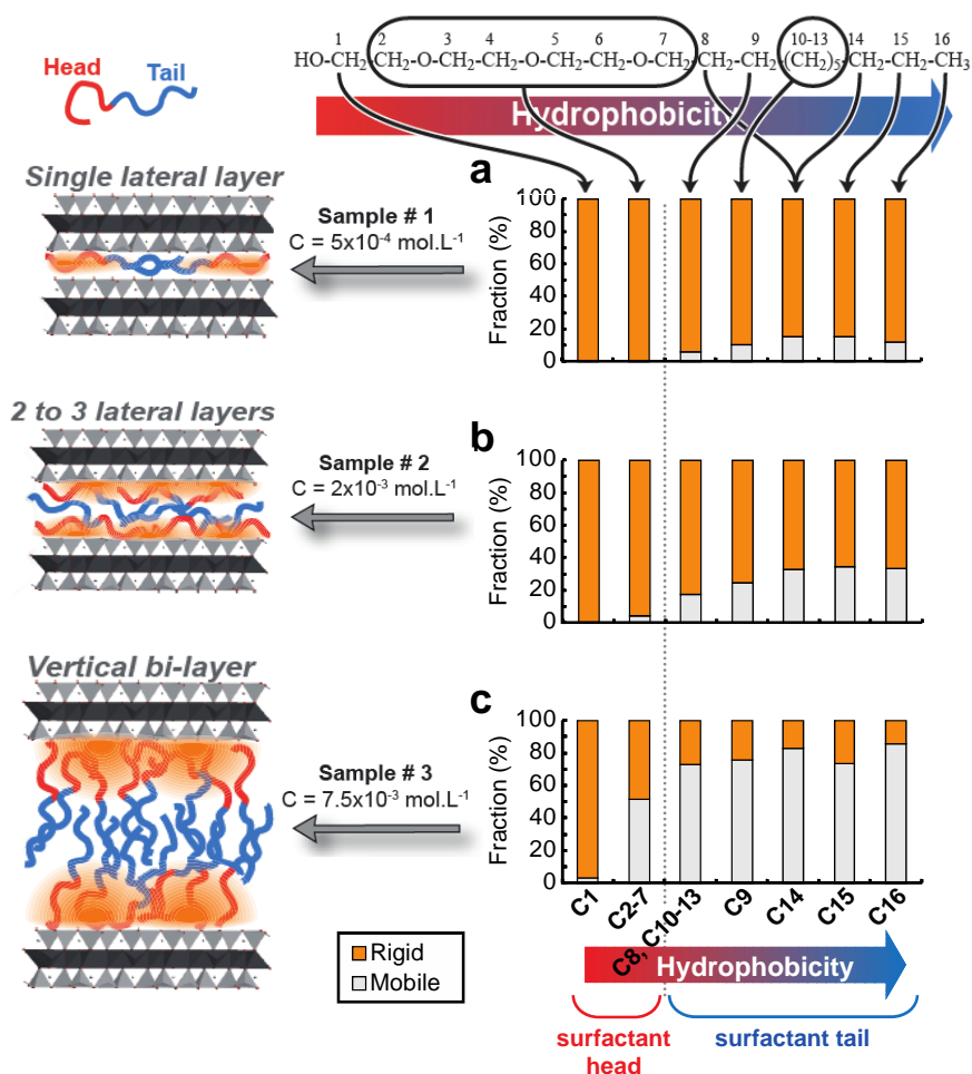
Figure 5. Fractions of (orange) rigid and (pale gray) mobile carbon sites measured from quantitative 13 C NMR spectra for Mt-C 10 E 3 organoclay samples # (a) 1, (b) 2, and (c) 3 prepared with initial surfactant concentrations of 5 \times 10^{-4} , 2 \times 10^{-3} , and 7.5 \times 10^{-3} mol.L -1 , respectively.
