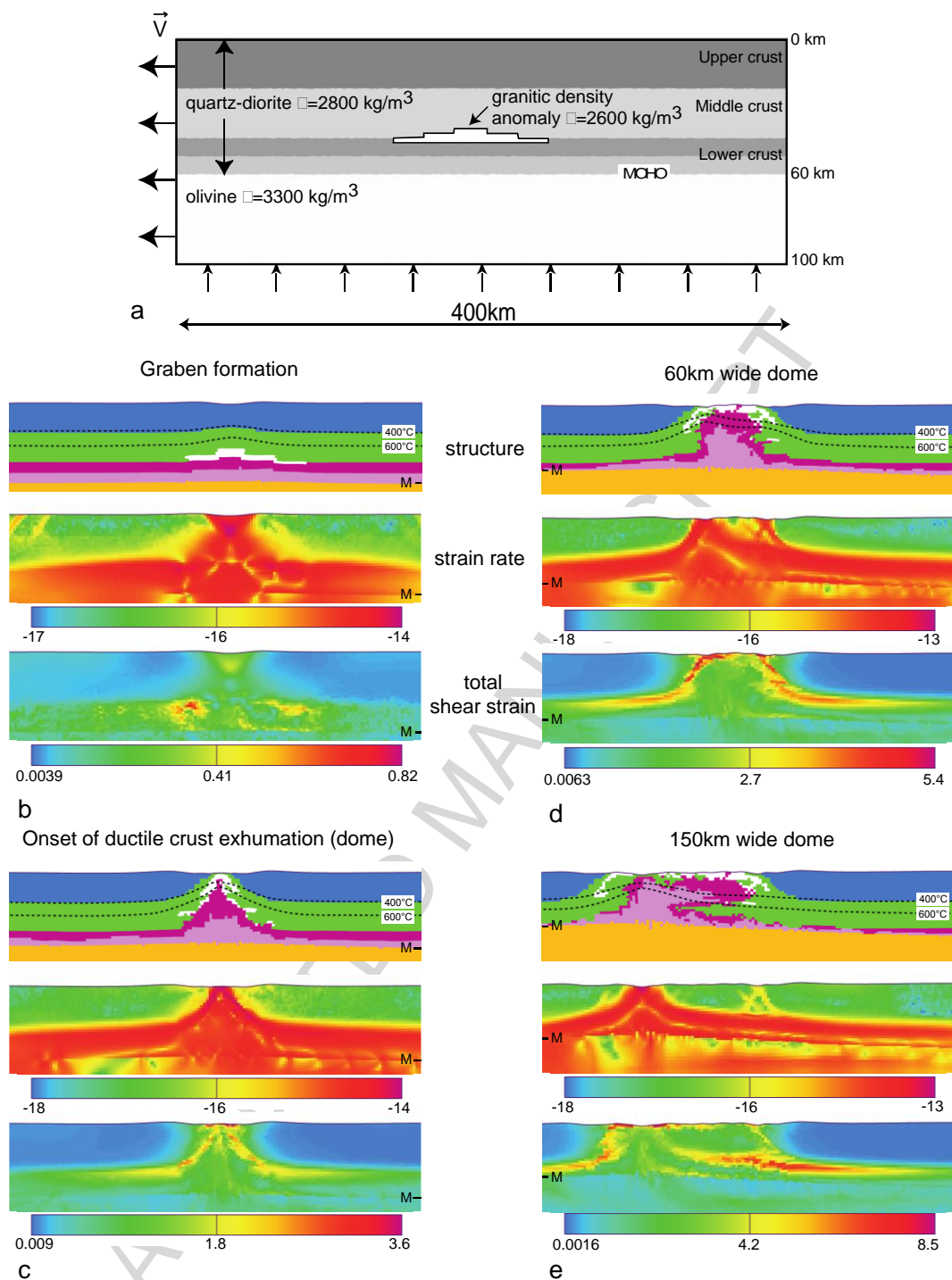
Fig.10. Numerical modeling of core complex development at lithosphere scale (modified from Tirel et al., 2008). a) Model geometry and velocity boundary conditions. b to d) Sections of models for increasing amount of extension. Each panel presents the model structure and the 400°C and 600°C isotherms (top section), the strain rate (middle section) and the pattern of total shear strain (down section). Structure, strain rate and total shear strain representations correspond to those parts of the computed numerical mesh where most of deformation is located and not to the entire initial model.
