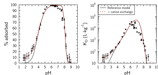
Fig. 10. Comparison of model predictions with U(VI) adsorption data of Pabalan and Turner (1996) . Cation exchange parameters are given in Table 3 . Solid concentration = 3.2 g·L -1 ; total U(VI) concentration = 2 \cdot 10^{-7} mol·L -1 . The results are presented in percentage adsorbed (left) and in log 10 K_D values (right) for a better evaluation of model fits at low (left) and high (right) U(VI) adsorption.
