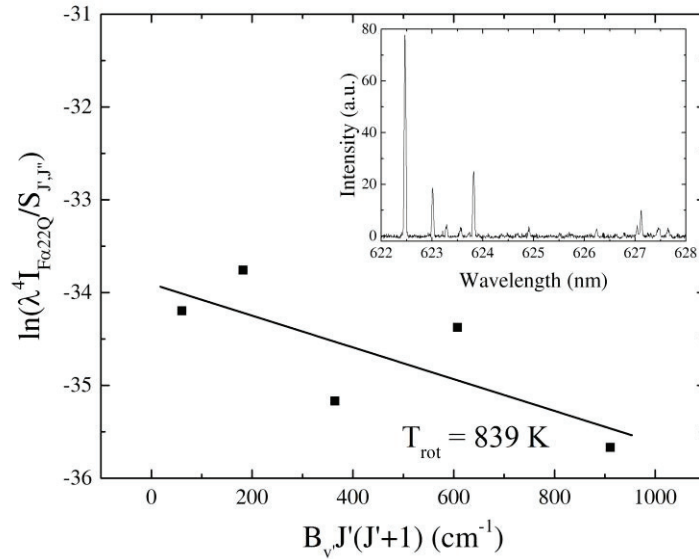
FIGURE 4. Boltzmann plot for the determination of the rotational temperature from the 2-2Q band of the Fulcher- \alpha system. The inset presents the corresponding spectrum. This specific measurement has been realized previously under similar to the present experimental conditions.
