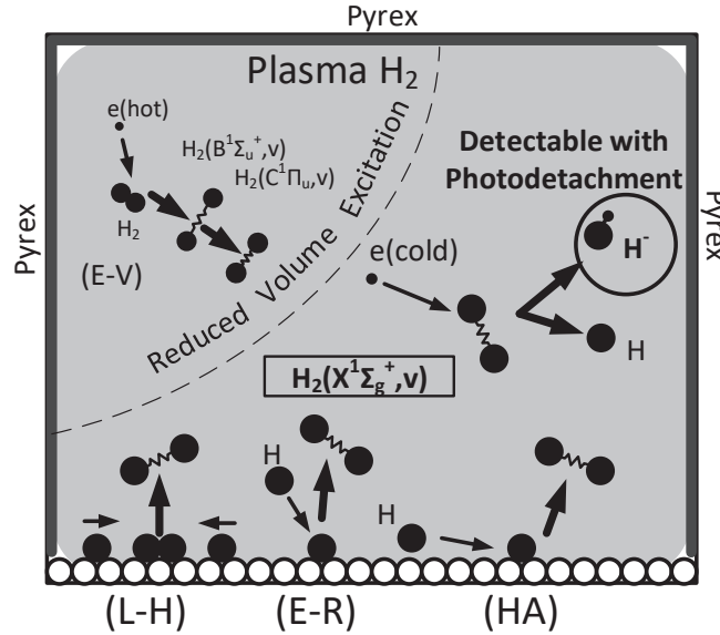
FIGURE 1. Concept of the source ROSAE III. The production of vibrationally excited molecules is limited as much as possible to the recombinative desorption on the surface of the material under test. L-H, E-R, and HA refer to the Langmuir-Hinshelwood, Eley-Rideal, and hot atom desorption mechanisms, respectively.
