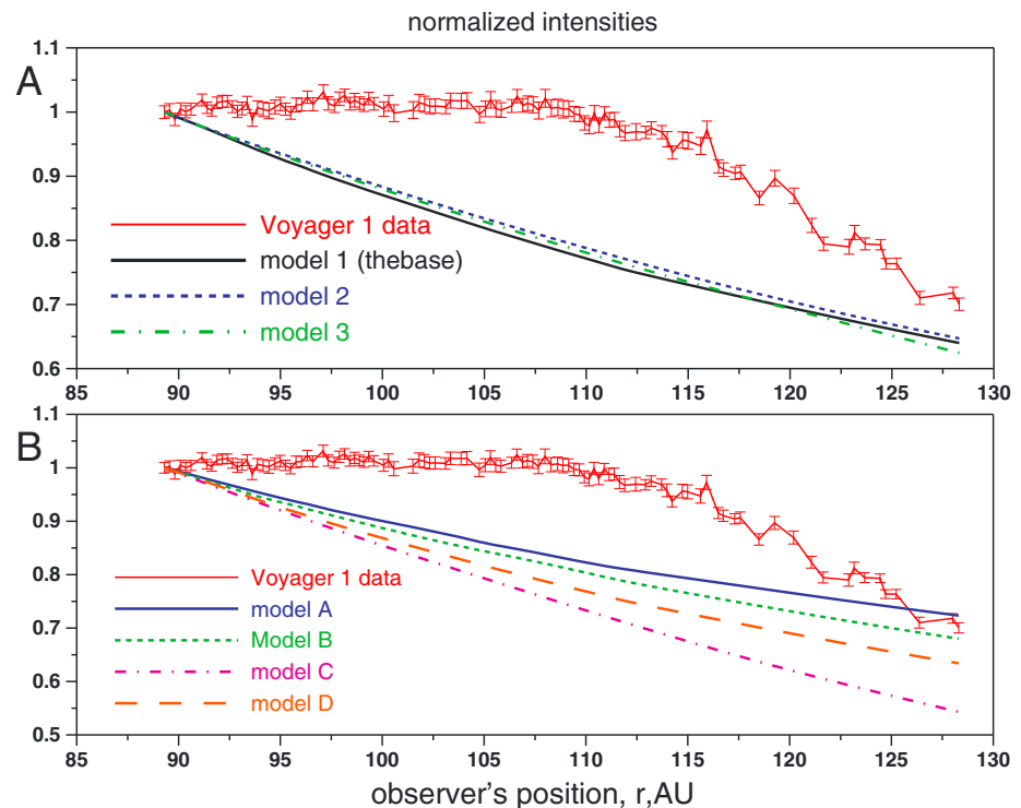
Figure 5. Comparison of the model results with Voyager 1/UVS data. All intensities are divided by the solar flux and normalized to unity at the first observational point (90 AU). (a) Results of three models with different LISM parameters (see Table 1). (b) Results of four test model calculations (A–D) are shown, see text for description of each test case.
