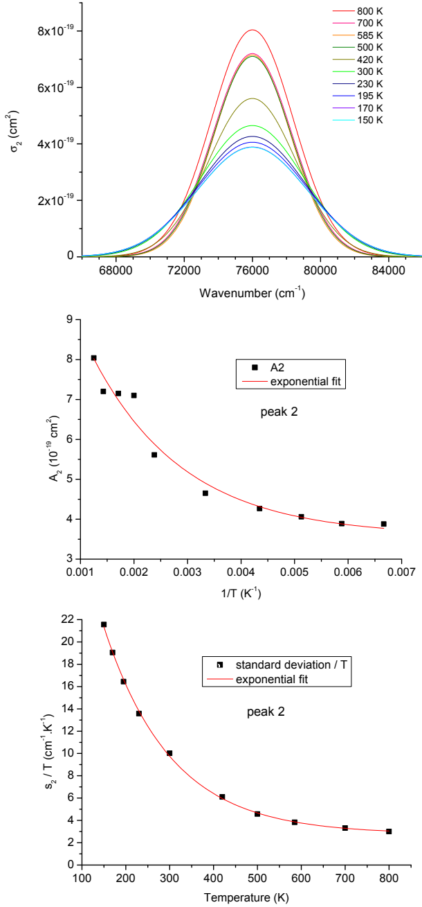
Fig. 4. Top: analytical representation of the second peak of \sigma_{\text{cont}}(\lambda, T) with a Gaussian function, \sigma_2(\lambda, T) , centred at 76\,000\text{ cm}^{-1} for temperatures between 150 and 800 K. Middle: variation of the amplitude A_2(T) of the second Gaussian function as a function of 1/T . The variation can be fitted by a decreasing exponential function. Bottom: variation of the standard deviation s_2(T)/T of the second Gaussian function as a function of the temperature. The variation can be fitted by a decreasing exponential function.
