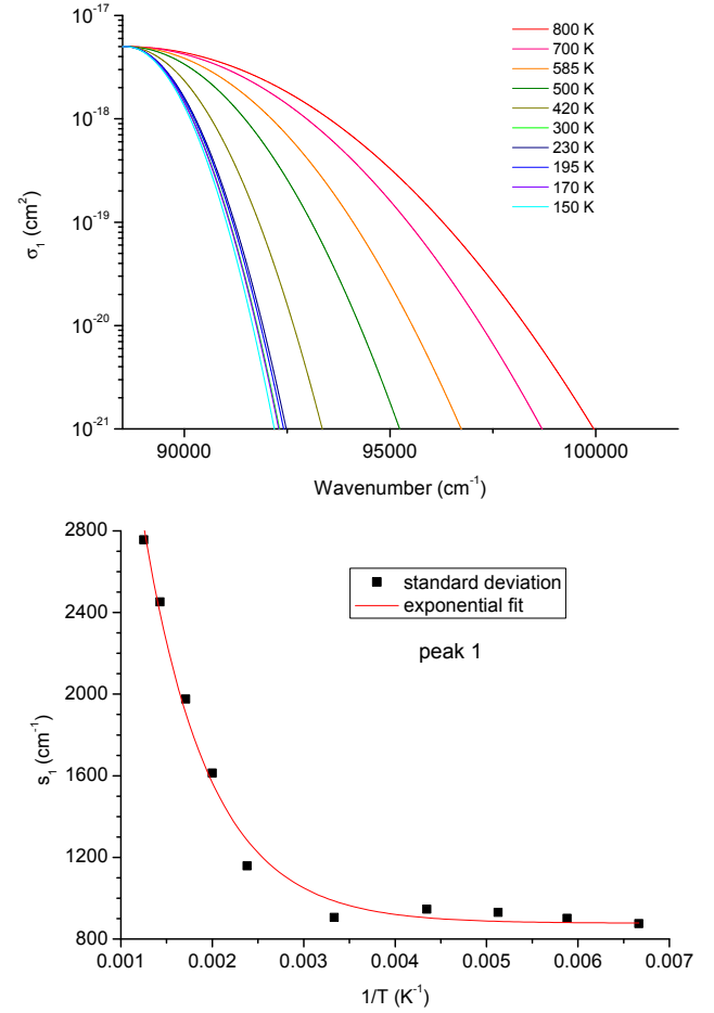
Fig. 3. Top: analytical representation of the first peak of \sigma_{\text{cont}}(\lambda, T) with a Gaussian function, \sigma_1(\lambda, T) , centred at 88\,574 cm -1 for temperatures between 150 and 800 K. Bottom: variation of the standard deviation s_1(T) of the first Gaussian function as a function of 1/T . The variation can be fitted by a decreasing exponential function.
