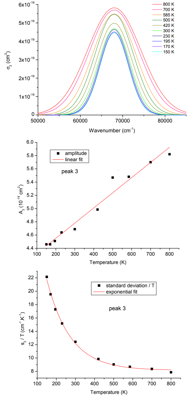
Fig. 5. Top: analytical representation of the third peak of \sigma_{\text{cont}}(\lambda, T) with a Gaussian function, \sigma_3(\lambda, T) , centred at 68\,000 \text{ cm}^{-1} for temperatures between 150 and 800 K. Middle: variation of the amplitude A_3 of the third Gaussian function as a function of the temperature. The variation can be fitted by a linear function. Bottom: variation of the standard deviation s_3(T)/T of the third Gaussian function as a function of the temperature. The variation can be fitted by a decreasing exponential function.
