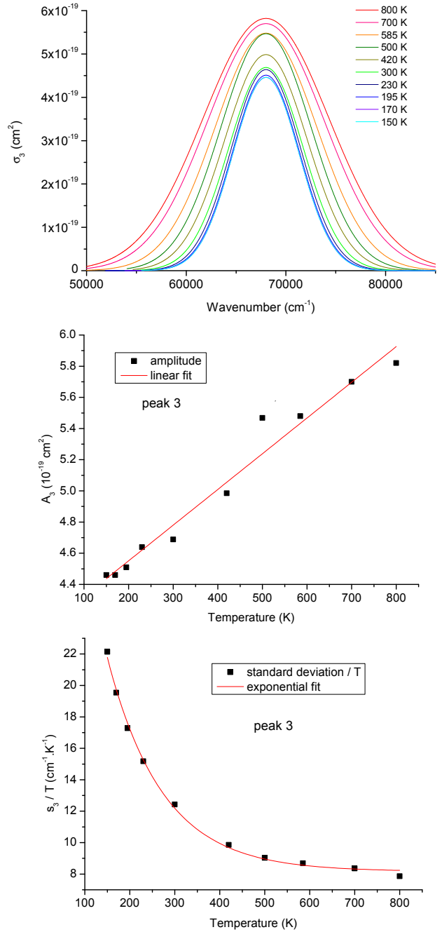
Fig. 5. Top: analytical representation of the third peak of \sigma_{\text{cont}}(\lambda, T) with a Gaussian function, \sigma_3(\lambda, T) , centred at 68 000 \text{cm}^{-1} for temperatures between 150 and 800 K. Middle: variation of the amplitude A_3 of the third Gaussian function as a function of the temperature. The variation can be fitted by a linear function. Bottom: variation of the standard deviation s_3(T)/T of the third Gaussian function as a function of the temperature. The variation can be fitted by a decreasing exponential function.
